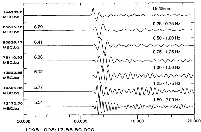
Fig. 7.4.5. Examples illustrating the multiple narrow-band filter technique for measuring m_b . For each plot, the largest m_b value would be selected as representing the station m_b . For station ASAR (top), the max "narrow-band" m_b is 5.56 (compared to analyst m_b of 5.67) and for station MBC (bottom) the corresponding numbers are 6.41 and 6.39. Thus, the correspondence is quite good in these two examples.
