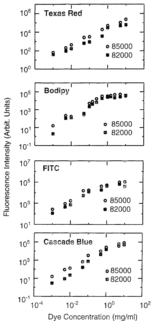
Fig. 2. Single dye emission vs. dye concentration. The emission intensity for TR, BD, FITC and CB were measured using both filter sets for concentrations of dye-BSA between 1 \mu\text{g}/\text{ml} and 10 mg/ml. Note the log-log scale. In most cases the relationship is linear over the majority of the concentration range. Detection limits are generally 1–10 \mu\text{g}/\text{ml} of dye.
