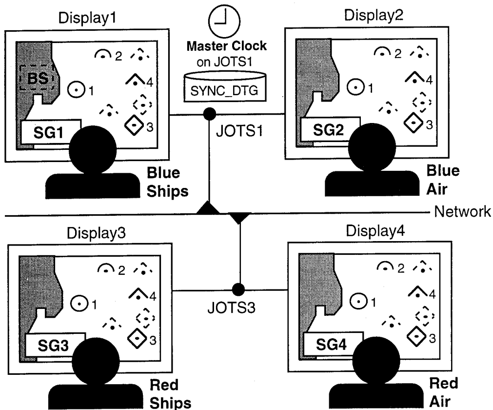
Fig. 14 — Multiple Scenario Generators for team training
