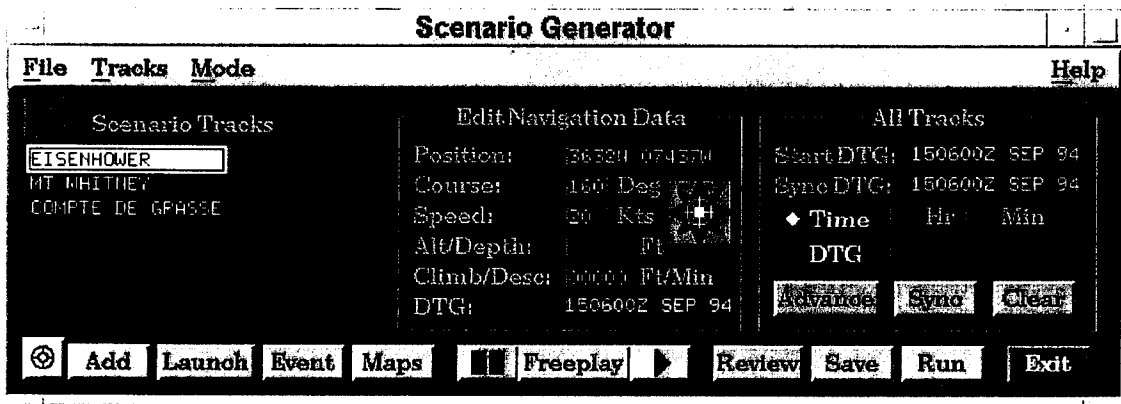
Fig. 8 — Scenario Generator Main Application window
