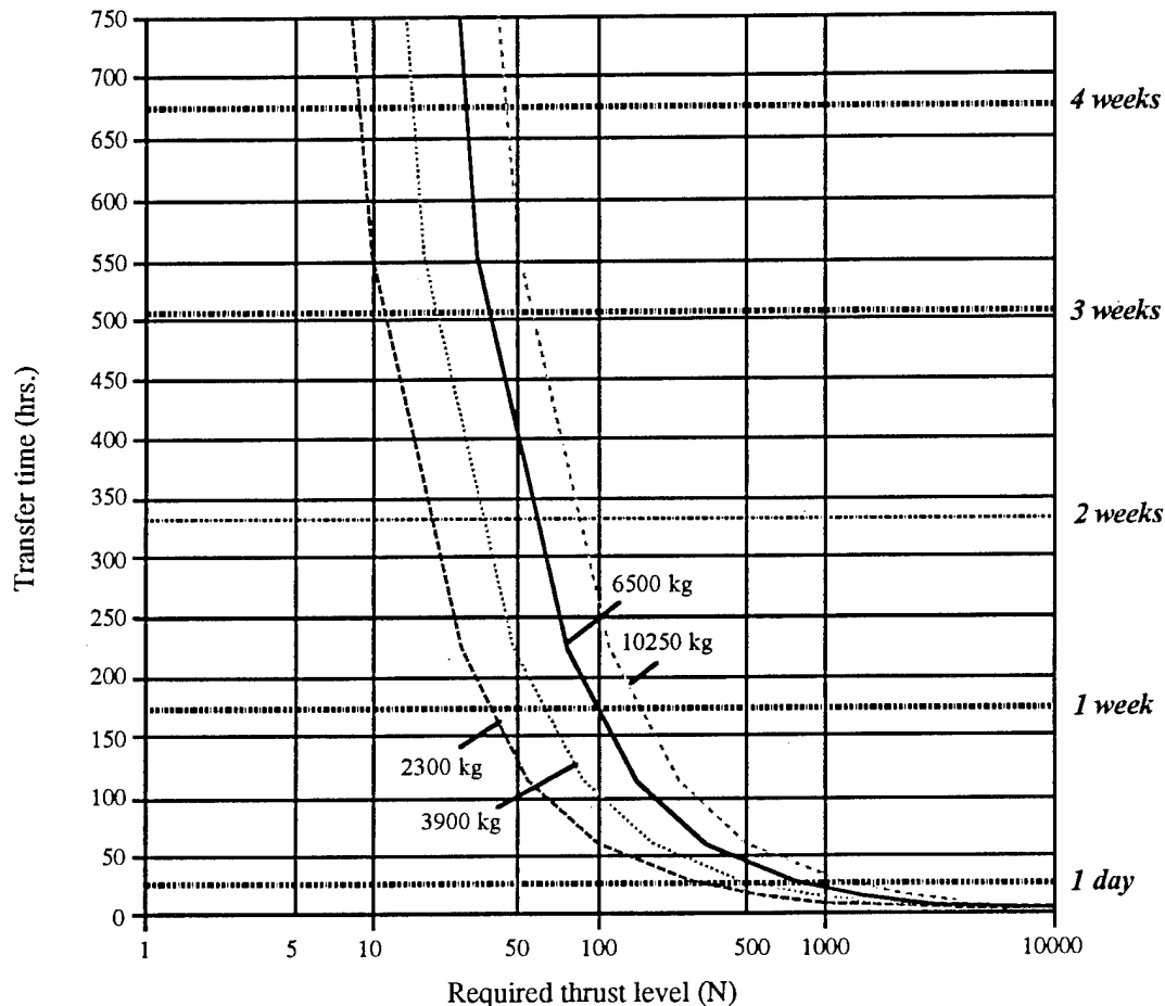
Thrust level requirement for various LEO-GEO transfer times from 1 day to 4 weeks (GEO payload masses of 2300, 3900, 6500, and 10250 kg)
