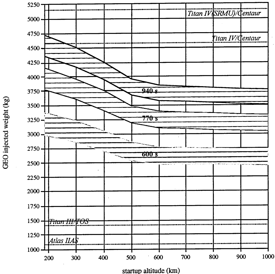
Figure 3.11 The range of injected weights for a given altitude and I_{sp} correspond to the performance of low thrust-to-weight ( \sim 10^{-4} ) and high thrust-to-weight ( \sim 1 ).
