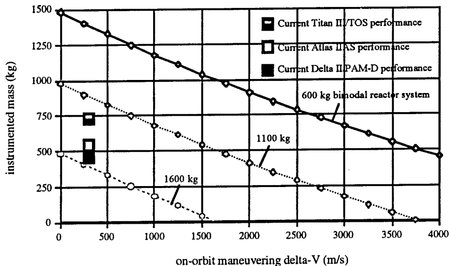
Figure 4.9 Assumptions are the same as in the previous chart. The bimodal system achieves a specific impulse of 940 s ( H_2 exhaust temperature of approximately 3000 K).
