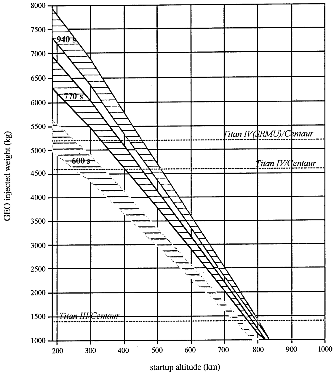
Figure 3.12 The range of injected weights for a given altitude and I_{sp} correspond to the performance of low thrust-to-weight ( \sim 10^{-4} ) and high thrust-to-weight ( \sim 1 ).
