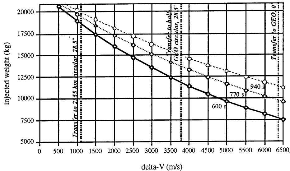
Figure 3.24 Assumptions for this chart include a launch from ETR into a 185-km circular parking orbit, a bimodal reactor system operating at a thrust-to-weight of 10^{-4} , and a variable I_{sp} (600, 770, and 940 s).
