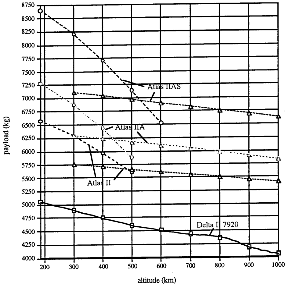
Figure 3.2 Assumptions are the same as in the previous figure (28.5° inclination, circular orbit). The payload capability of these systems degrade fairly gracefully at higher altitudes. There are two sets of performance curves for each booster, corresponding to a single Centaur burn (higher payloads at low altitudes) and a two-burn (curves beginning at 300 km).
