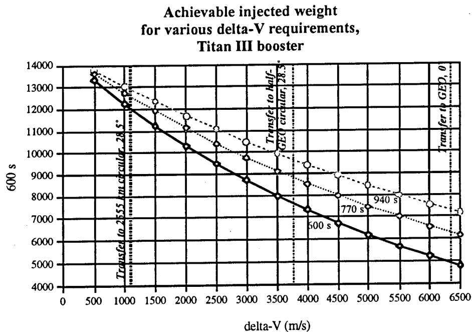
Figure 3.23 Assumptions for this chart include a launch from ETR to a 185-km circular parking orbit, a bimodal reactor system operating at a thrust-to-weight of 10^{-4} , and a variable I_{sp} (600, 770, and 940 s).
