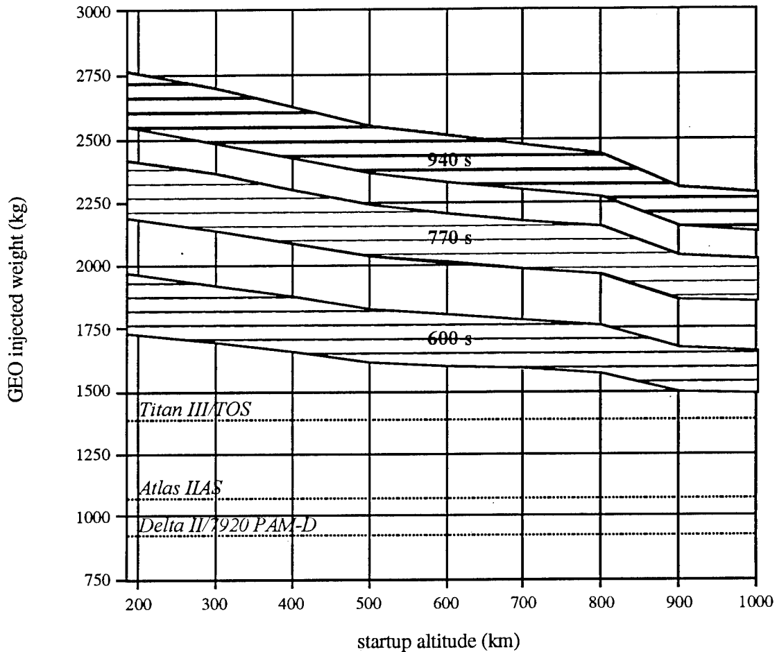
Figure 3.10 The Delta II/7920 payload capability to low altitudes is fairly flat. The broken lines for Delta II/7920 PAM-D, Atlas IIAS, and Titan III/TOS represent current maximum payload deliveries to GEO. The range of injected weights for a given altitude and Isp correspond to the performance of low thrust-to-weight ( \sim 10^{-4} ) and high thrust-to-weight ( \sim 1 ).
