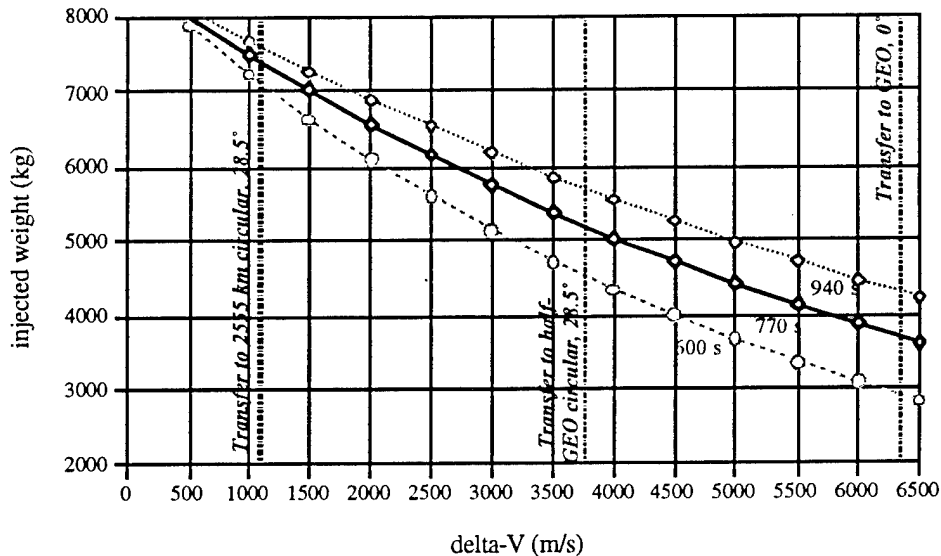
Figure 3.22 Assumptions for this chart include a launch from ETR into a 185-km circular parking orbit, a bimodal reactor system operating at a thrust-to-weight of 10^{-4} , and a variable I_{sp} (600, 770, and 940 s).
