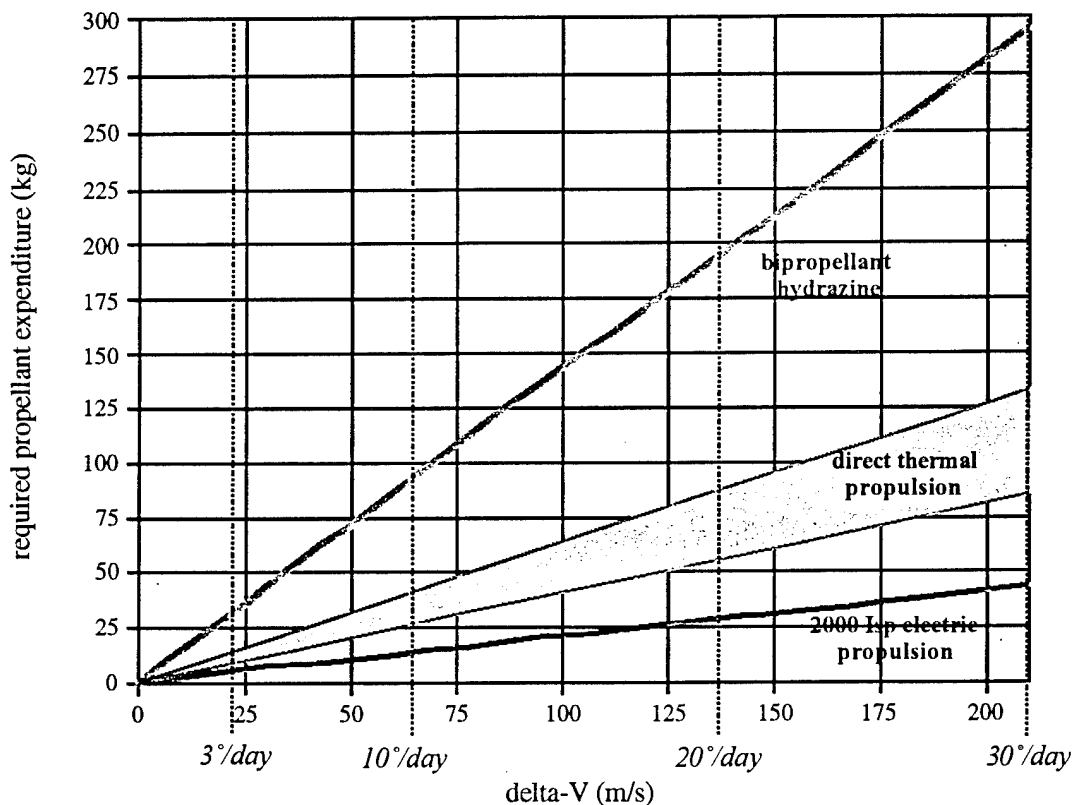
Figure 3.20 Direct nuclear thermal propulsion cuts propellant consumption by approximately a factor of three. Using high-performance electric propulsion (2000 s) would reduce overall consumption by a factor of six or more.
