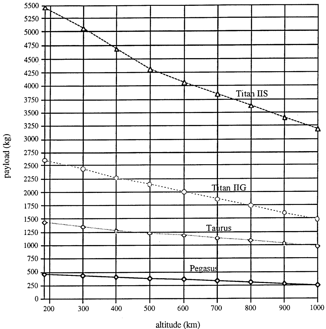
Figure 3.1 Assumptions include launch from Cape Canaveral (ETR) into a 28.5° circular orbit and a Titan II launch capability at ETR (which does not currently exist). Titan IIS is an upgraded Titan configuration that is included for comparison purposes only, since the system is not currently operational.
