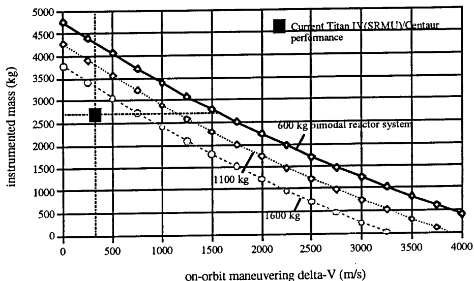
Figure 4.6 This chart displays the performance envelope of a bimodal satellite launched from a Titan IV(SRMU)/NUS and compares it to the current estimated capability of Titan IV(SRMU)/Centaur. The bimodal system achieves a specific impulse of 600 s ( H_2 exhaust temperature of approximately 1215 K). Dotted lines are provided to determine (1) increased maneuver capability for a fixed mass, and (2) increased instrumented payload for a fixed delta-V budget.
