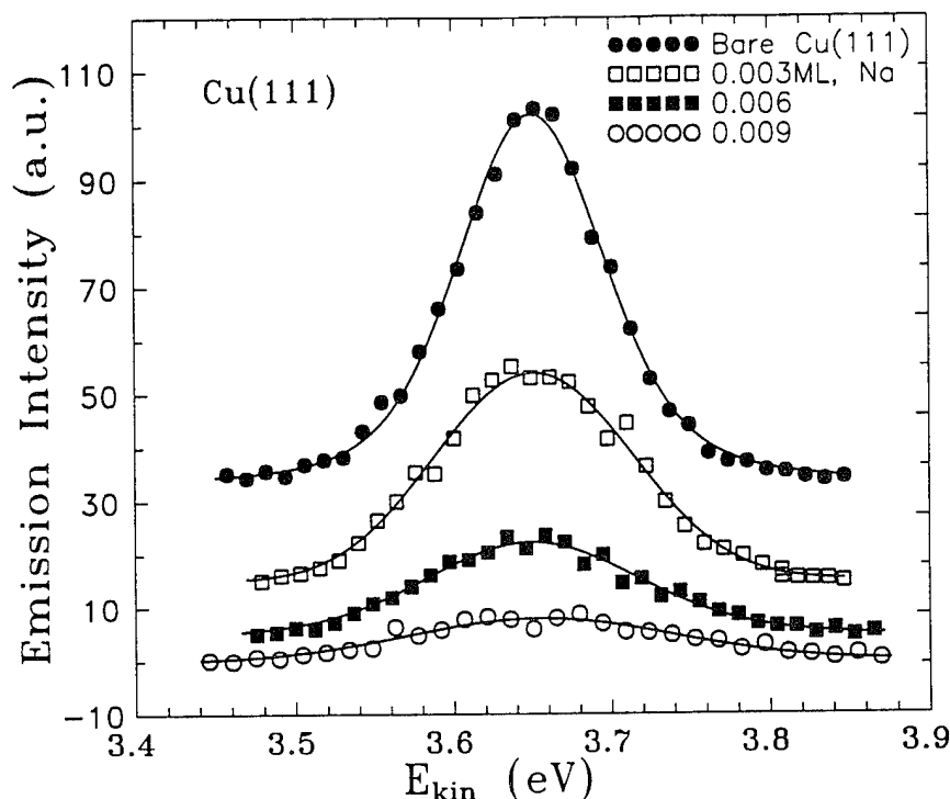
Figure 11. EDC's from the n = 1 image-state at normal emission from Cu(111) in the presence of Na adsorbate, at coverages of \Theta = 0, 3/1000, 6/1000, and 9/1000 ML, respectively. The fit to the data was obtained by a convolution of a Gaussian and a Lorentzian lineshape as described in the text, using a nonlinear least-square algorithm.
