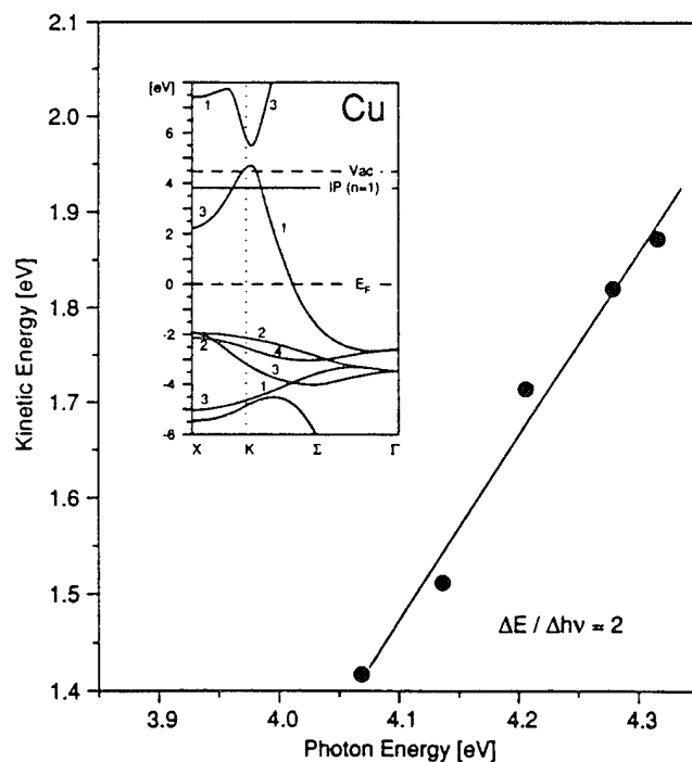
Figure 4. Variation of the kinetic energy of the 3d bulk band peak with change in photon energy. The \Delta E_{\text{kin}}=2\Delta h\nu dependence indicates a fixed initial state. The inset shows the bulk energy bands of Cu. 45,47,48
