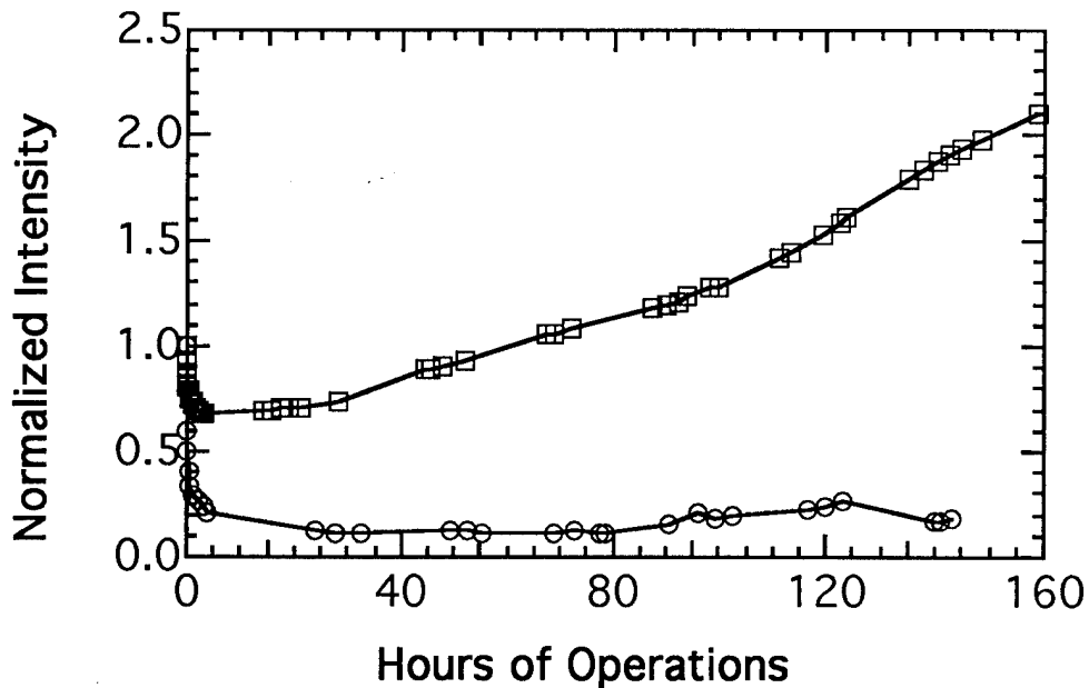
Figure 4: Time dependence of emission at \lambda=1.3 \text{ }\mu\text{m} for 55 \text{ }\mu\text{m} wide junction structure. Device was continuously operated at 10 \text{ mA} (circles) and 20 \text{ mA} (squares) constant current under ambient conditions.
