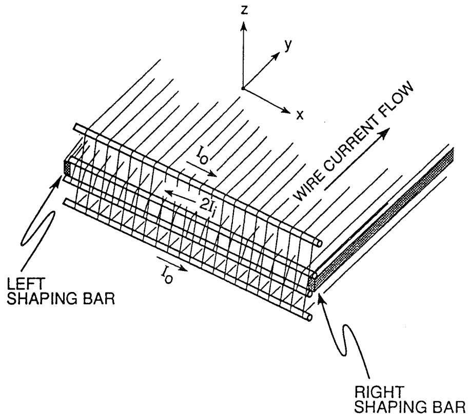
Grid showing shaping bars, feeder bar current directions, and orientation. z is along chamber z axis. Feeder bars are not shown.
