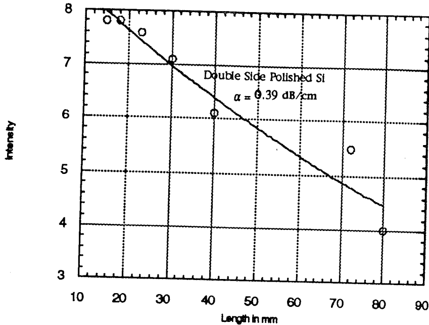
Figure 5: Output coupled intensity of Si substrate modes for samples of different length.
