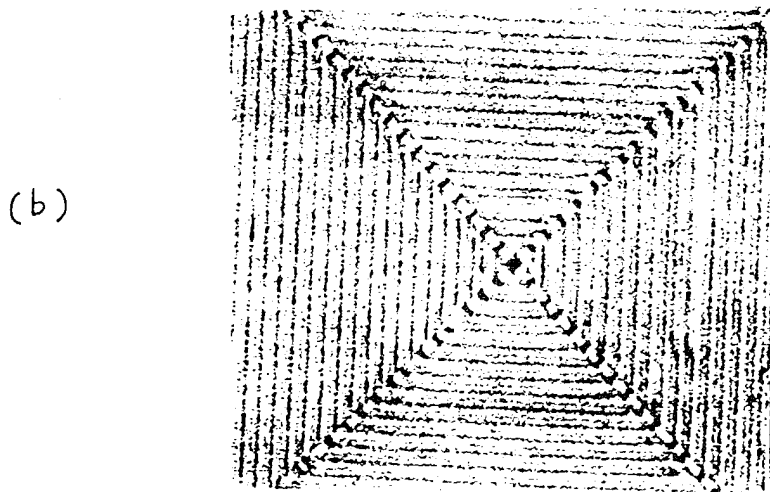
Figure 3a: Microscope photograph of the 2\ \mu\text{m} period input coupling hexagonal grating structure in silicon used to create a 1 to 6 fanout in the substrate. 3b: 1\ \mu\text{m} period square grating structure used to create the 1 to 4 fanout in the prototype device of figure 2
