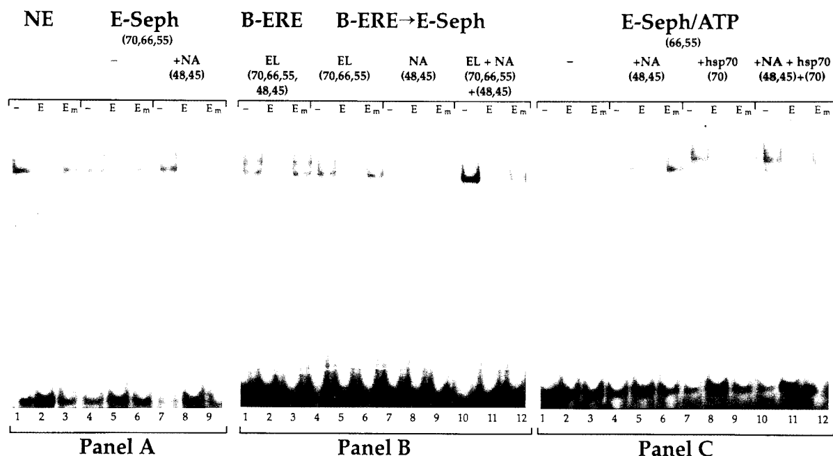
Fig. 6. Electrophoretic Mobility Shift Analysis of hER/ 32 P-ERE Interactions in the Presence or Absence of hER-Associated Proteins hER complexes were incubated for 30 min at 25 C with 32 P-labeled vitellogenin A2 ERE (27-mer) and electrophoresed on a 5% nondenaturing polyacrylamide gel. The source and composition of each mixture are outlined in Fig. 1. E and E m indicate the addition, respectively, of excess unlabeled vitellogenin A2 ERE (AGGTCAcagTGACCT) or a mutant ERE containing a 2-bp inversion (AGGTCAcagTGCACT). Panel A, CHO-ER nuclear extract (NE) (lanes 1–3), E-Septh eluate (lanes 4–6), E-Septh eluate + p48/p45 (B-ERE to E-Septh nonadsorbed [NA]; lanes 7–9). Panel B, B-ERE eluate (lanes 1–3), B-ERE to E-Septh eluate (lanes 4–6), NA (lanes 7–9), B-ERE to E-Septh eluate + NA (lanes 10–12). Panel C, E-Septh/ATP eluate (lanes 1–3), E-Septh/ATP eluate + NA (lanes 4–6), E-Septh/ATP eluate + hsp70 (lanes 7–9), E-Septh/ATP eluate + NA + hsp70 (lanes 10–12).
