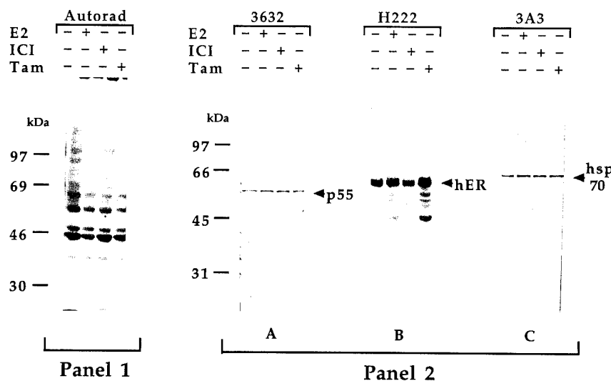
Fig. 4. Comparison of hER-Associated Proteins Isolated by DNA-Affinity Chromatography after Treatment of CHO-ER Cells with No Ligand, Estradiol, ICI-182,780, or OH-Tam during [ ^{35} S]Methionine Labeling
