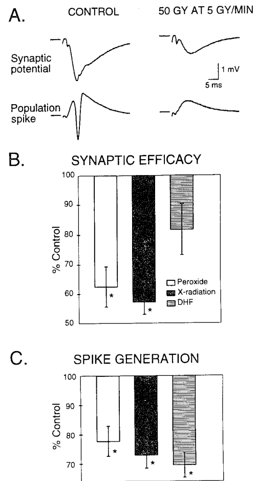
Fig. 1. Synaptic efficacy and spike generation are reduced by free radicals. A: sample field potential recordings obtained from field CA1 of guinea pig hippocampal slice before and after exposure to 50 Gy X-radiation at a dose rate of 5 Gy/min. The synaptic response to stimulation of stratum radiatum was significantly decreased by the radiation. The resulting population spike was completely blocked by the exposure. B: reduction in synaptic efficacy by hydrogen peroxide (3 mM), X-radiation (50 Gy at 5 Gy/min) and dihydroxyfumarate (3 mM). The effects of dihydroxyfumarate were not statistically significant. C: reduction in spike generation by hydrogen peroxide (3 mM), X-radiation (50 Gy at 5 Gy/min) and dihydroxyfumarate (3 mM). The effects reflect the decreased ability of constant size synaptic potential to elicit a population spike. n = 9 for peroxide, n = 4 for X-radiation, n = 7 for dihydroxyfumarate. * reflects significance at P < 0.05\% .
