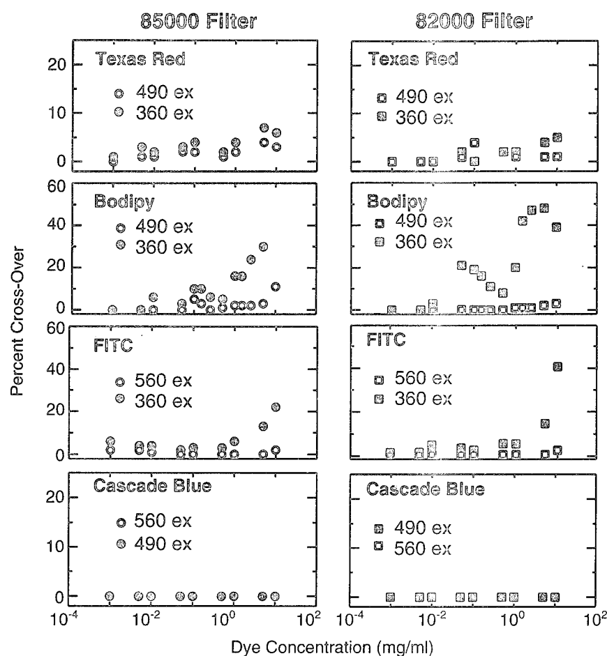
Fig. 3. Filter cross-talk characteristics with single dyes. Cross-talk for dye concentrations between 1 \mu\text{g/ml} and 10 mg/ml were measured for both the 85000 (left panels) and 82000 (right panels) filters for TR, BD, FITC and CB. Values for both non-optimum wavelengths are presented in each panel. The values are the percentage emission for each dye that is excited by wavelengths other than the optimum for that dye normalized to the dye's reported excitation maximum. For Texas Red the optimum excitation filter was 560 nm and the two non-optimum wavelengths are 360 and 490 nm. For most dye, filter and wavelength combinations, cross-talk is less than 10% of the maximal emission obtained at the dye's excitation maximum. BD and FITC at 360 nm and at high concentrations showed much higher levels.
