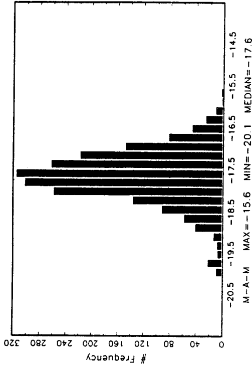
WSMR Log C_N^2 at 12.1 km N=2057 (9 months: 91:M-A-M 92:M-M 93:M-A-M 94:A)
