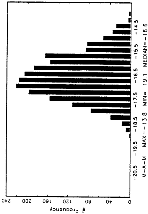
WSMR Log C_N^2 at 5.6 km N=2057 (9 months: 91:M-A-M 92:M-M 93:M-A-M 94:A)
