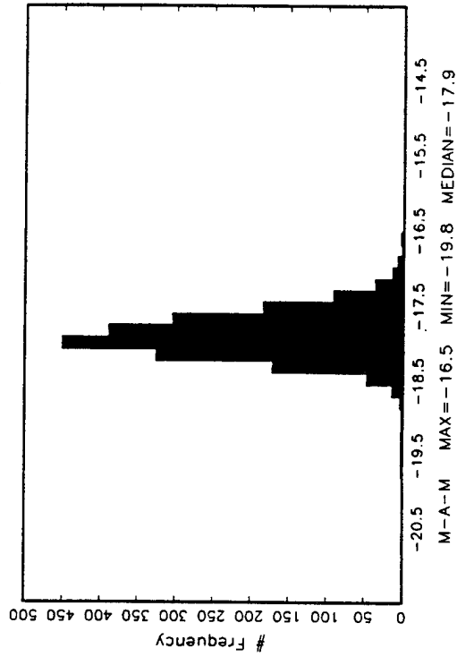
WSMR MEDIAN Log C_N^2 at 12-18 km N=2057 (9 months: 91:M-A-M 92:M-M 93:M-A-M 94:A)
