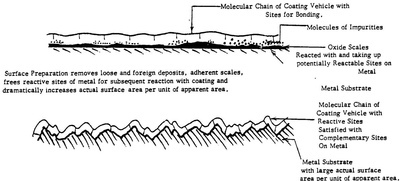
Figure 15-1. Surface Preparation
