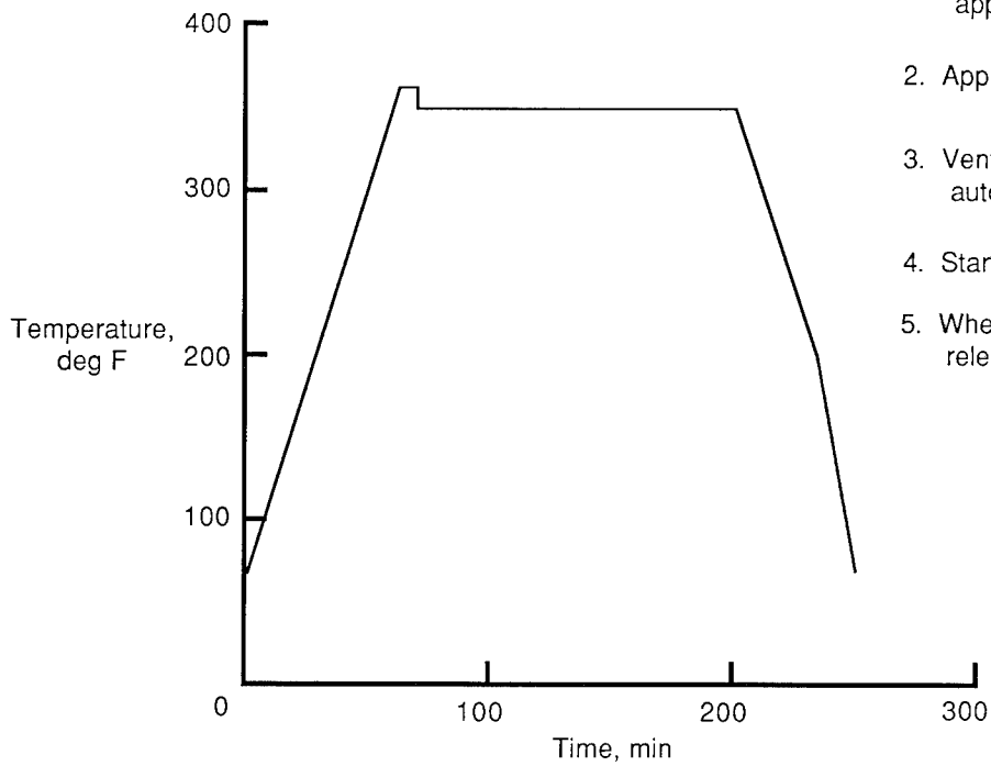
Figure 3. Standard cure cycle.
