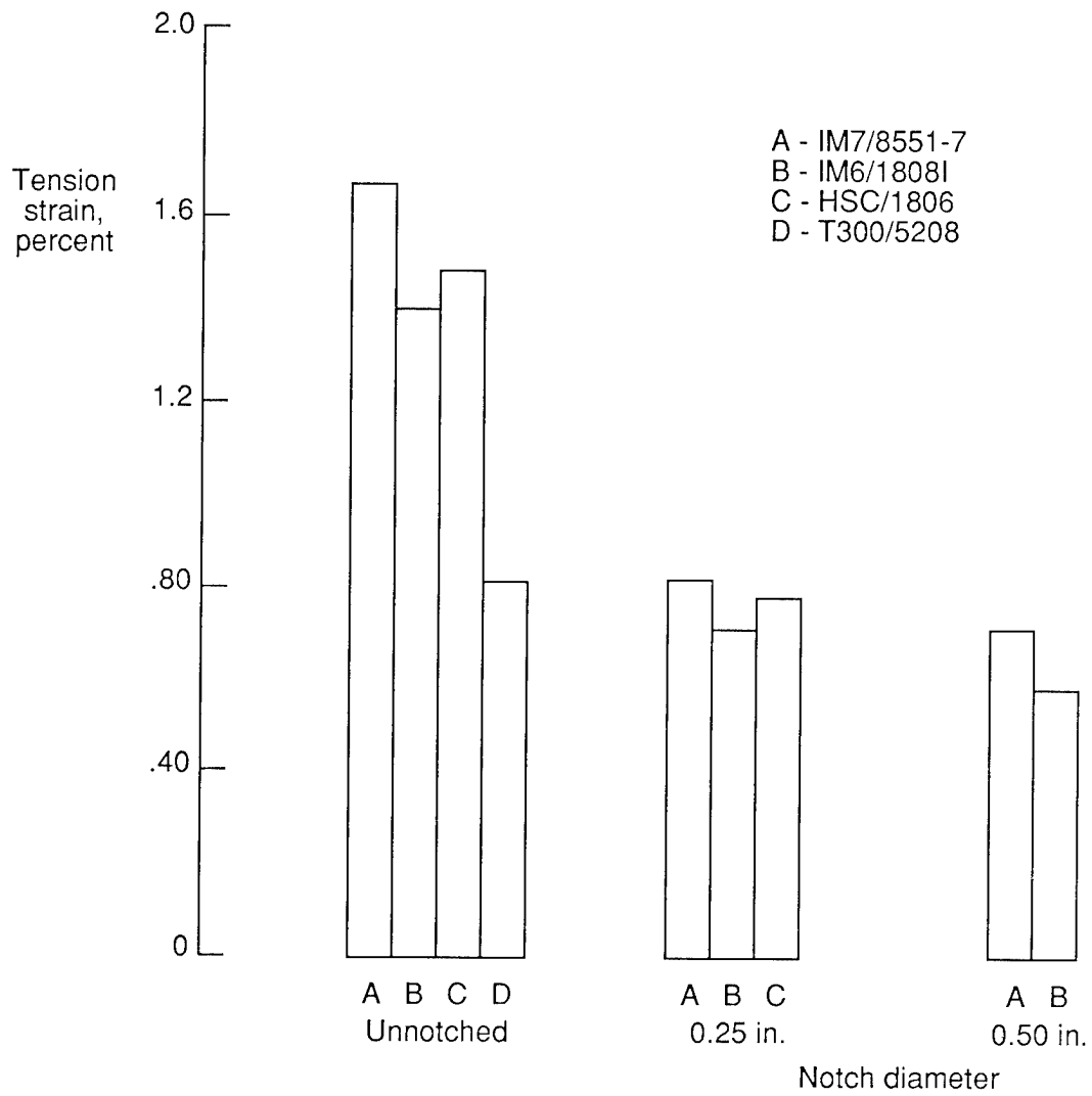
(b) Tension failure strain.
