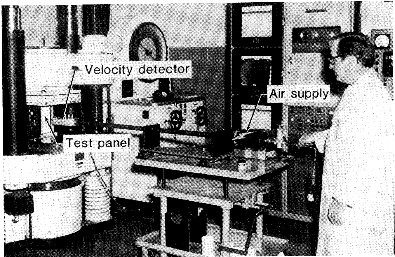
Figure 7. Impact test apparatus.
