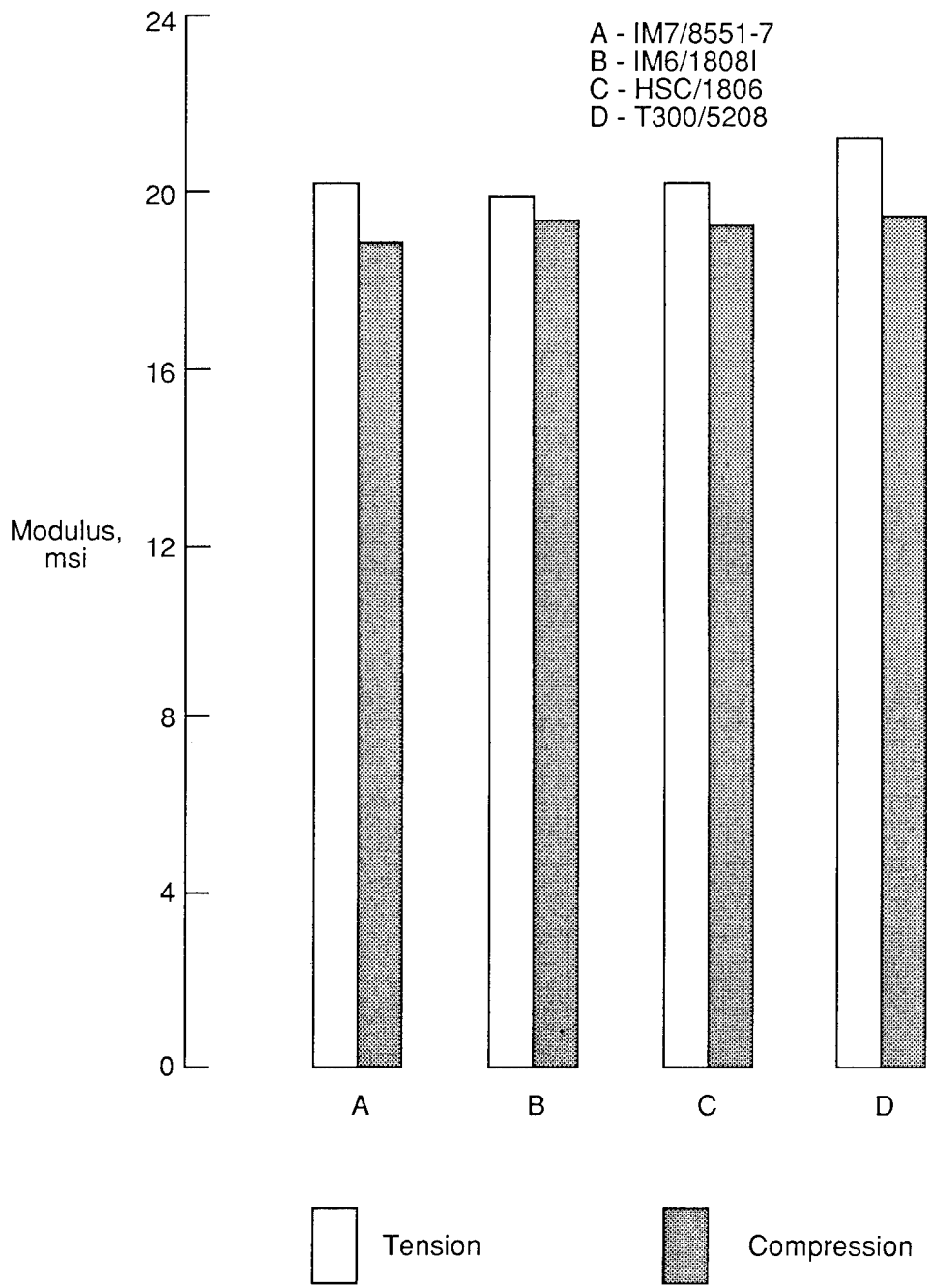
(b) Tension and compression moduli.
