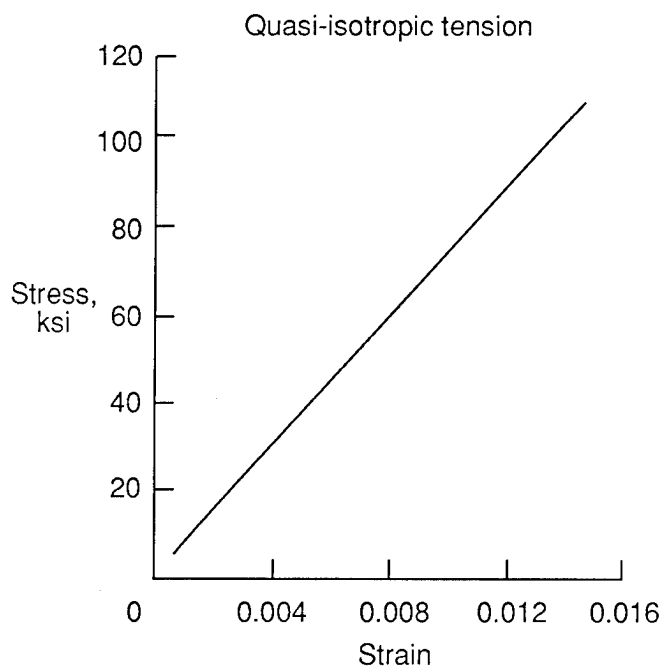
Figure 10. Typical stress-strain curves for IM6/1808I laminates.
