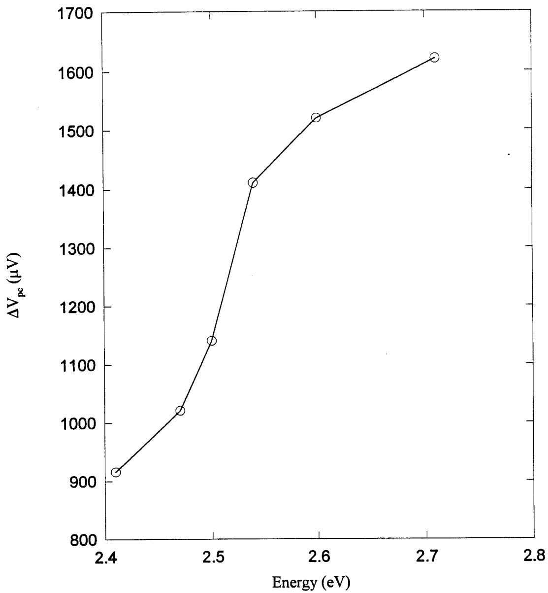
Figure 14. Photoconductivity of Ca_{0.34}:YIG
