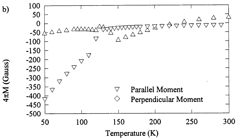
Figure 10. Temperature Dependence of the Magnetization in zero applied field for an a) annealed sample and b) unannealed Sample of \text{Bi}_{0.8}\text{Tm}_{2.14}\text{Pb}_{0.06}\text{Ga}_{1.9}\text{Fe}_{3.1}\text{O}_{12} .
