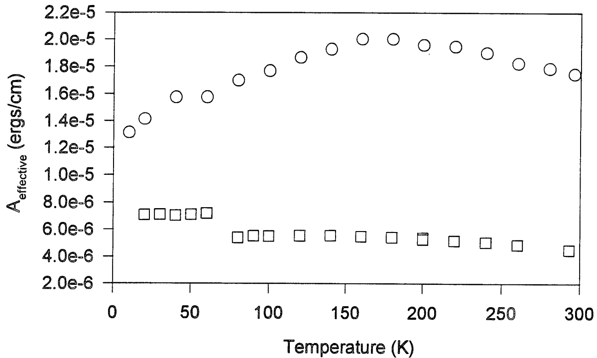
Figure 12. (a) The effective g-value and (b) the effective exchange constant of \text{Ca}_{0.24}\text{:YIG} for both an as-grown sample - ○ and a sample annealed in \text{N}_2 at 1000 C for 7 hours - □
