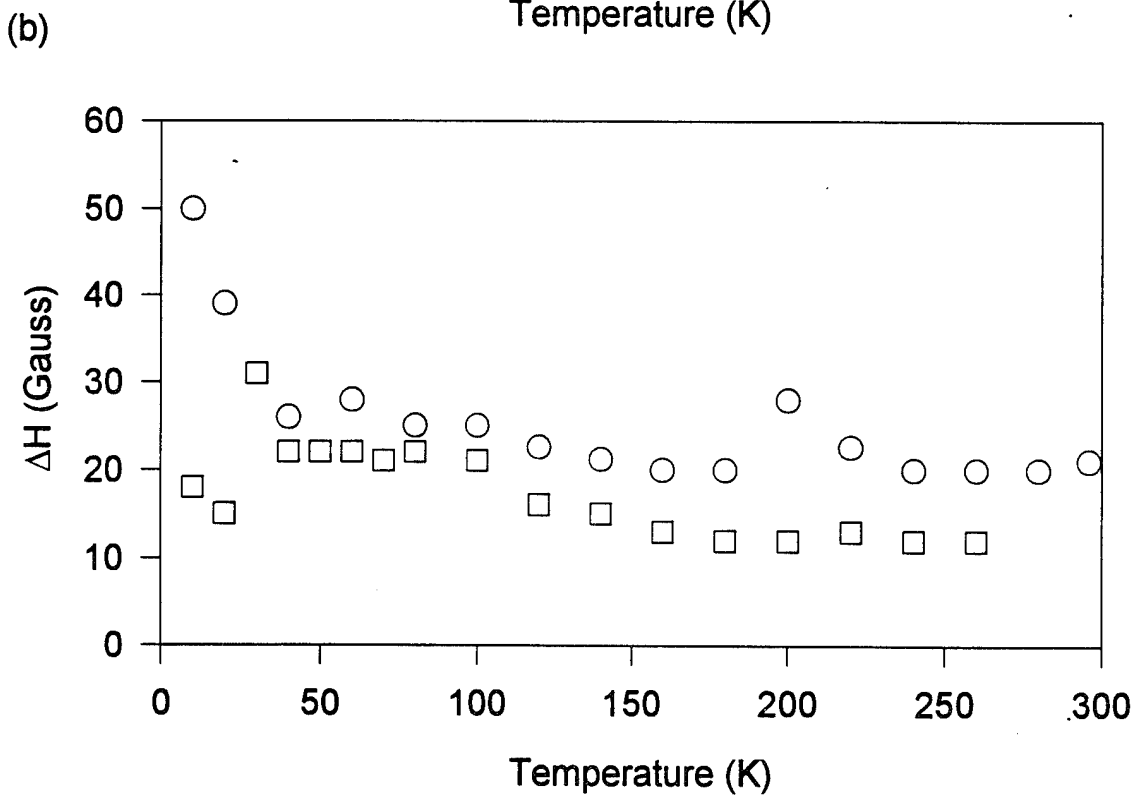
Figure 11. (a) The effective anisotropy field and (b) the in-plane FMR linewidth of \text{Ca}_{0.24}\text{:YIG} for both an as-grown sample - ○ and a sample annealed in \text{N}_2 at 1000 C for 7 hours - □
