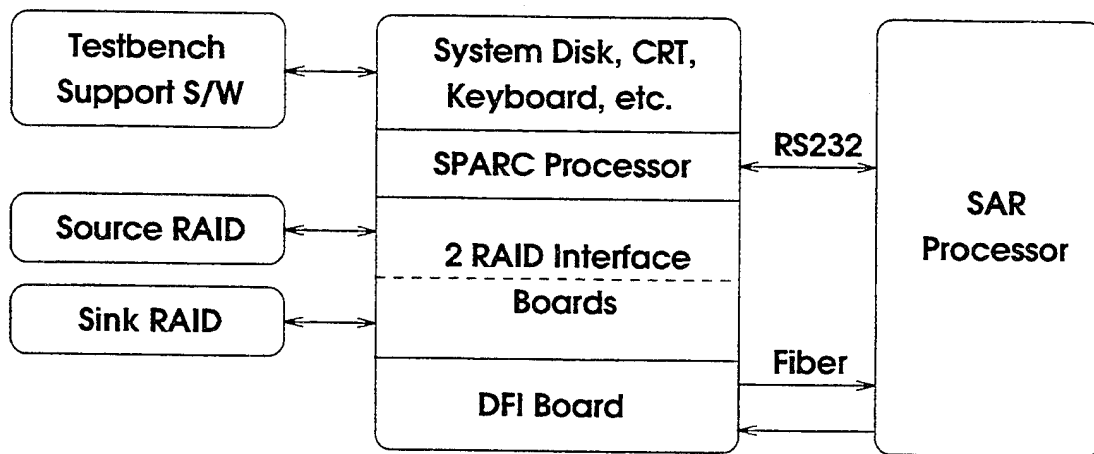
Figure 6. Basic test system layout.
