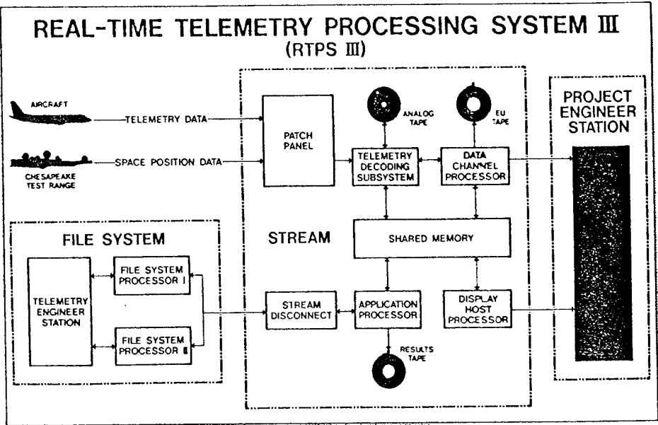
Figure 1. RTPS Architecture
