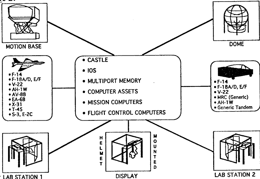
Figure 2. MFS Architecture
