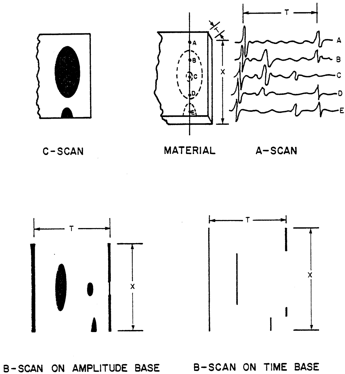
Figure 16. B-Scan Formation
