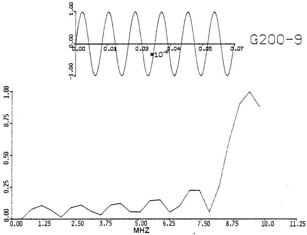
(a) 512-Point FFT of 6 Periods of 9 MHz Sine
