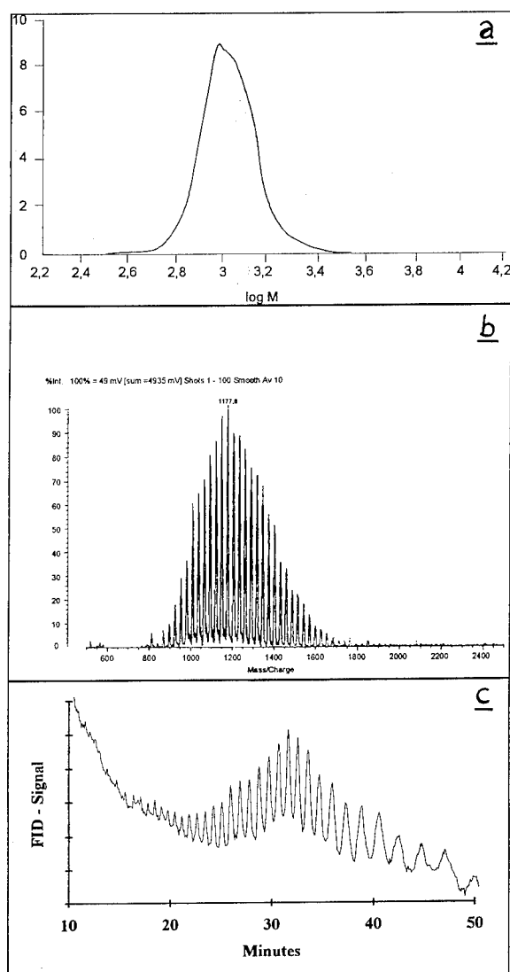
Fig.1: SEC-, SFC-chromatograms and MALDI mass spectrum of a technical wax ( M_w \sim 1000 \text{ Da} )
