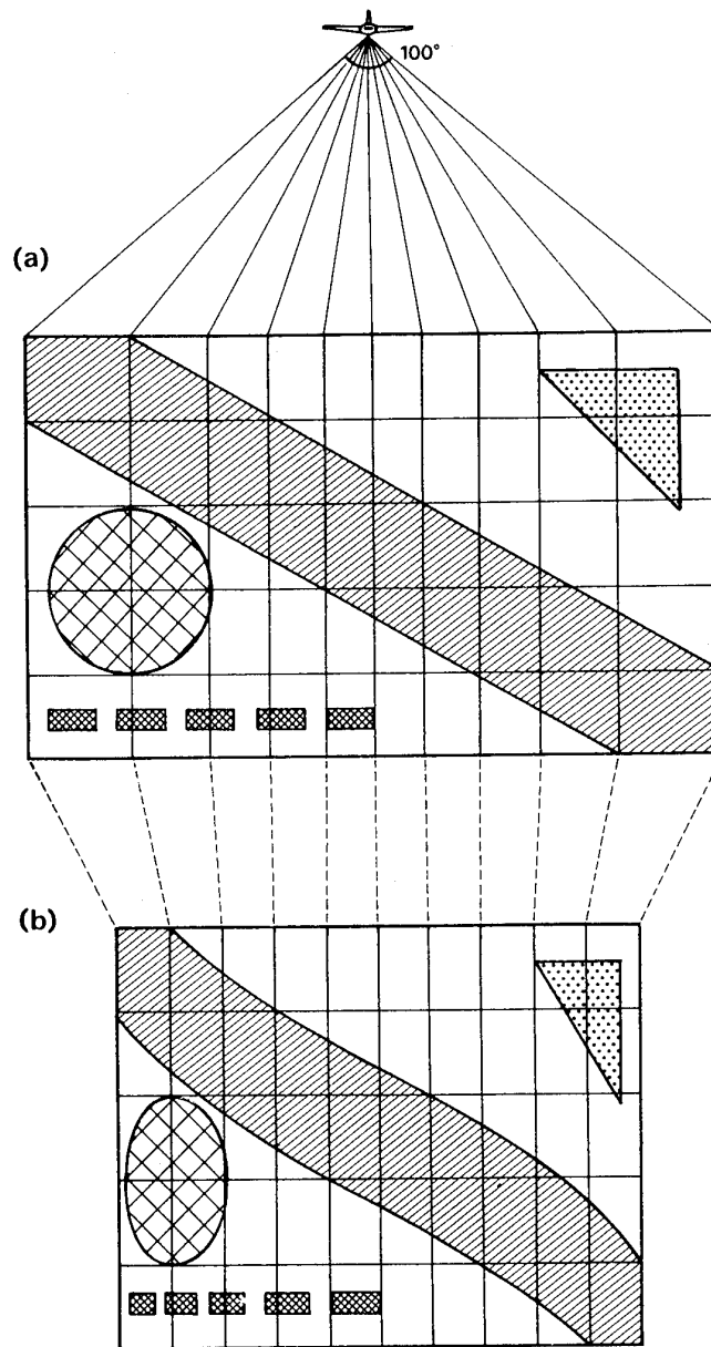
Figure 2. Effect of scan angle in aircraft imagery. a Panoramic distortion: pixel width increases significantly away from a vertical view. b Resulting image distortions: image features have lateral distortion when displayed with constant pixel width. Reproduced from Harrison and Jupp (1989)
