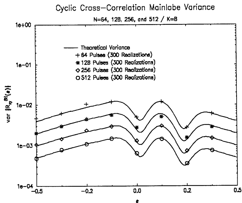
Figure 6.5. Average Realized Squared Error Functions and Expected Error Functions for N=64, 128, 256, and 512 Pulses.
