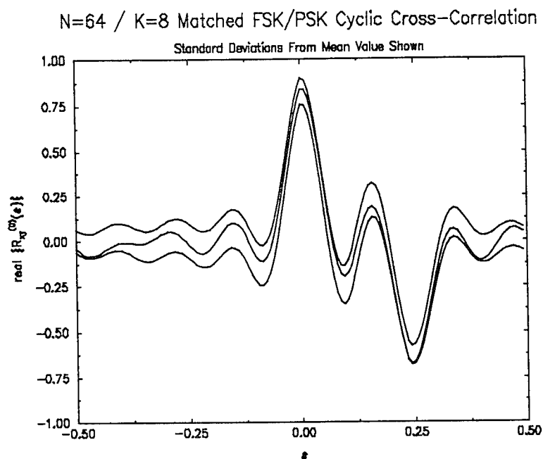
Figure 6.3.a. Real Component of the Realized Matched FSK/PSK Cross-Ambiguity Function and Standard Deviations for N=64 and K=8.
