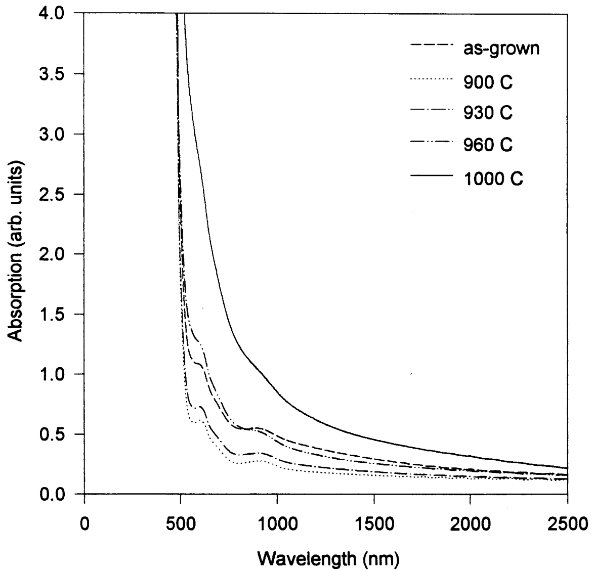
Figure 16. Optical absorption spectra of Ca 0.18 :YIG for a sample successively annealed at the indicated temperatures in a N 2 atmosphere.
