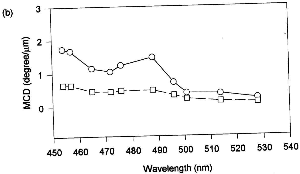
Figure 15. (a) The Faraday rotation and (b) the magnetic circular dichroism of \text{Ca}_{0.24}\text{:YIG} for both an as-grown sample - ○ and a sample annealed in \text{N}_2 at 1000\text{ }^\circ\text{C} for 7 hours - □
