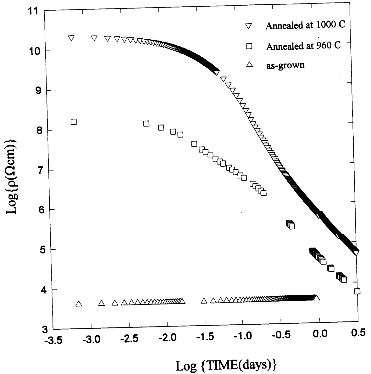
Fig. 5. The dependence of the resistivity decay process on different annealing conditions [E = 10^4 \text{ V/cm (100 V), } T = 300 \text{ K}]
