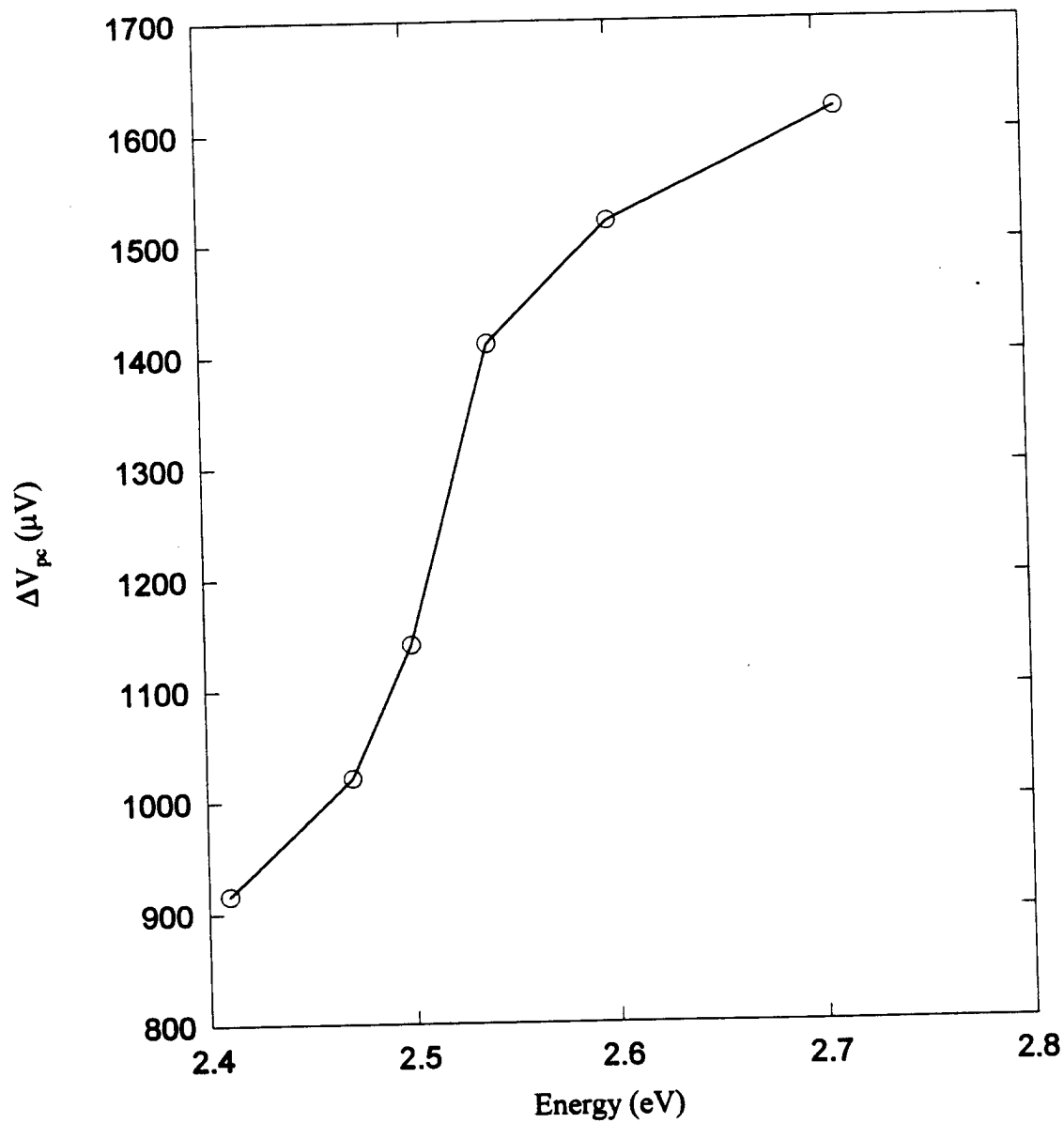
Figure 14. Photoconductivity of Ca_{0.34}:YIG
