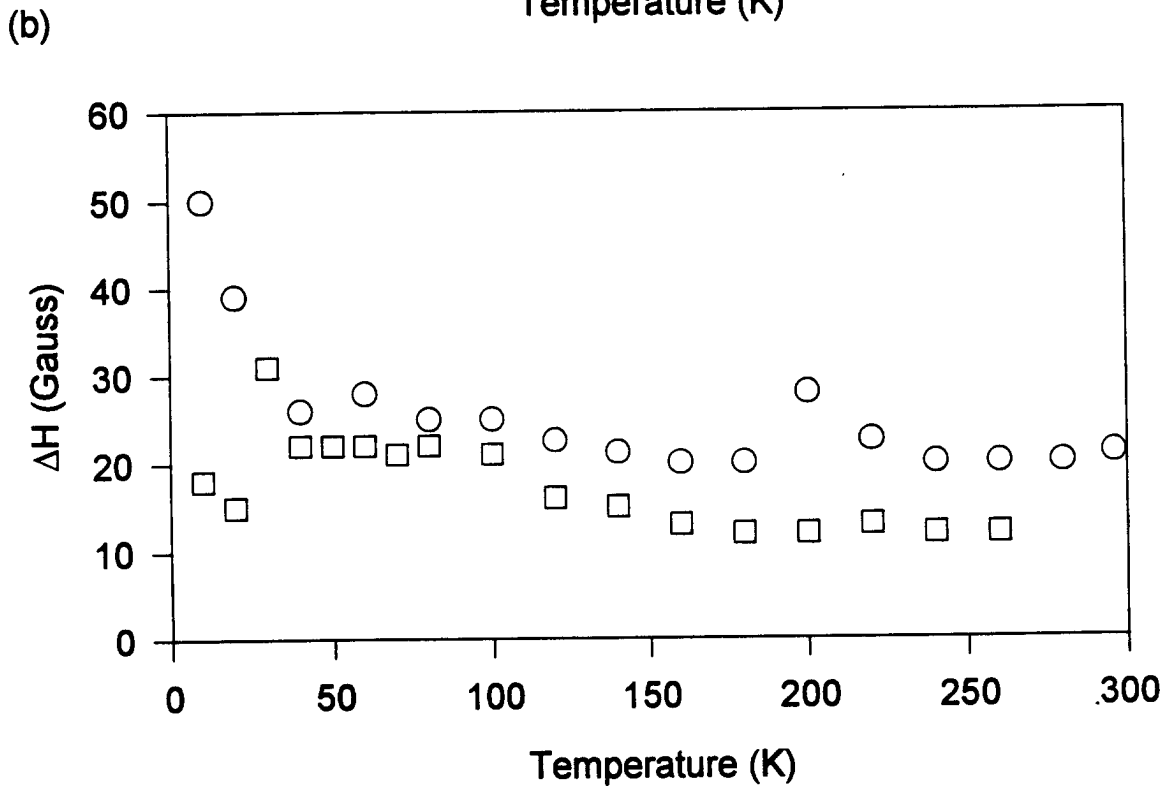
Figure 11. (a) The effective anisotropy field and (b) the in-plane FMR linewidth of \text{Ca}_{0.24}\text{:YIG} for both an as-grown sample - ○ and a sample annealed in \text{N}_2 at 1000 C for 7 hours - □
