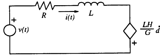
Figure 2: Magnetizing circuit model
