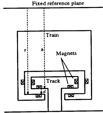
Figure 1: Cross section of a MLV train
