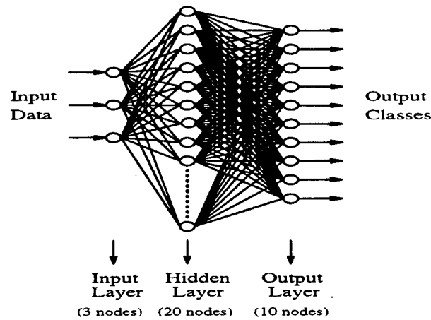
Figure 7: Network architecture of MLV system classifier
