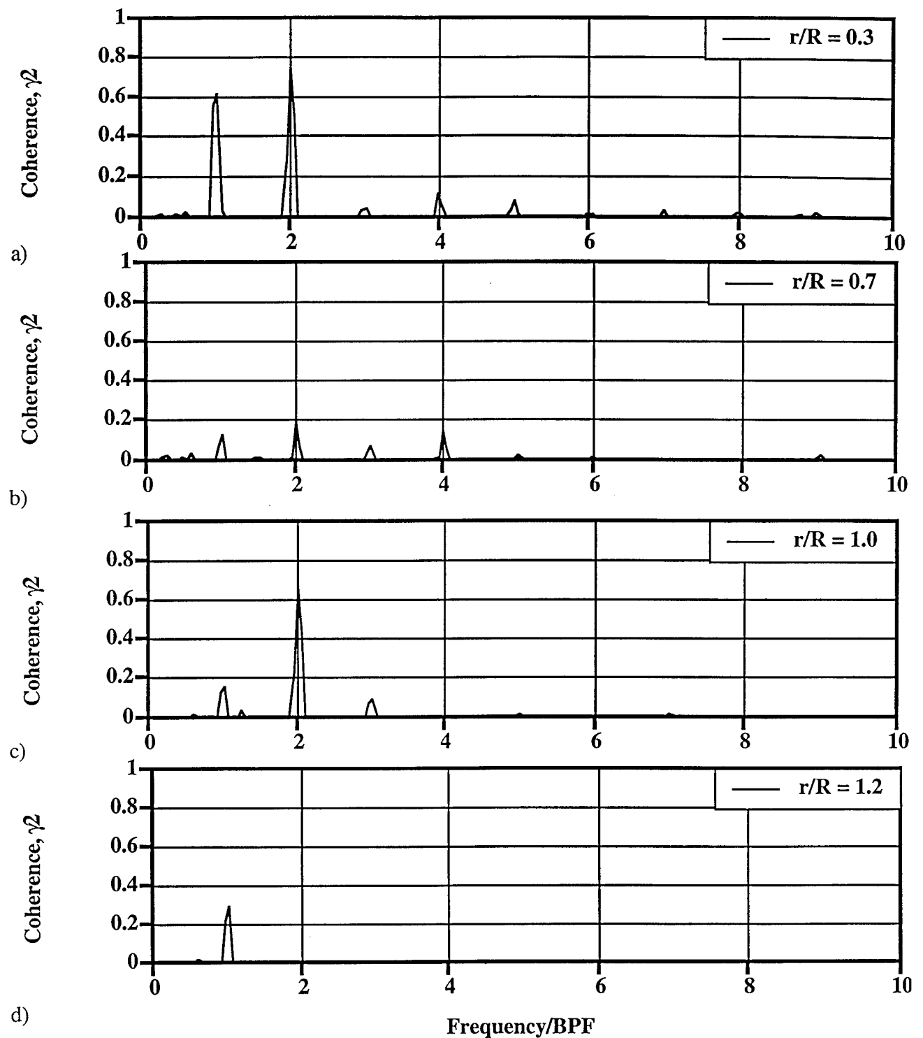
Figure 19. Coherence Function Spectra for Hot-Wire/Microphone Measurements with Turbulent Inflow from Grid m = 3 in., U_\infty = 33 ft/s, 3000 RPM, Microphone at r/R = 15 , \phi = 120^\circ , and Hot-Wire Locations in Propeller Wake at x/R = 0.025 and a) r/R = 0.3 , b) r/R = 0.7 , c) r/R = 1.0 , and d) r/R = 1.2
