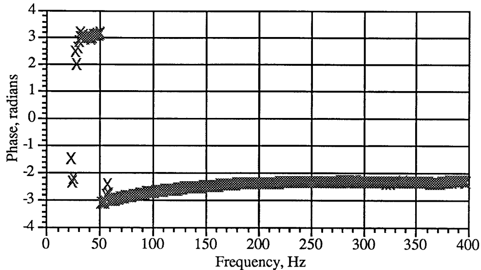
Figure 11 Phase difference between piezoelectric pressure transducer and 1/2" B&K microphone.
