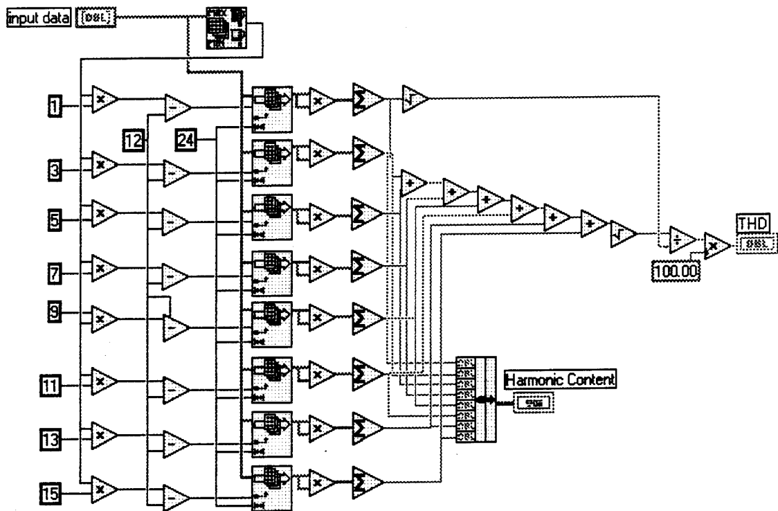
Figure 4.4 Block Diagram of THD subVI
