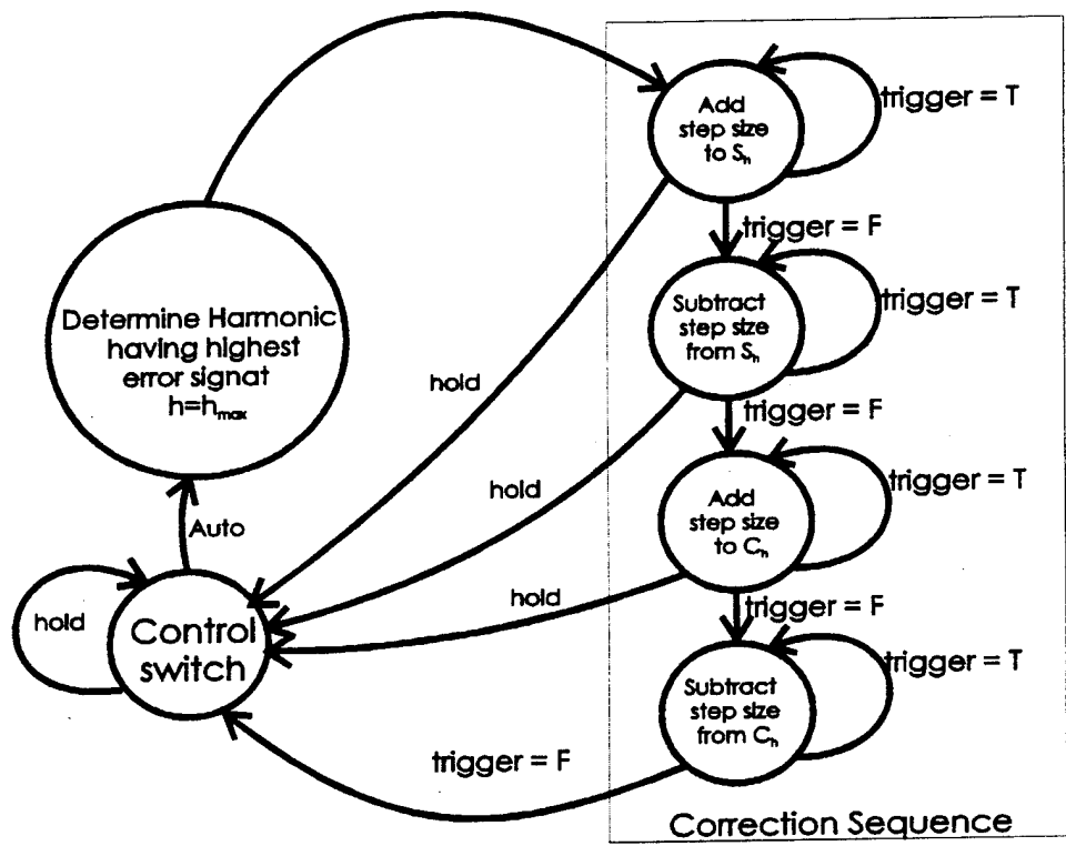
Figure 4.6 State Machine
