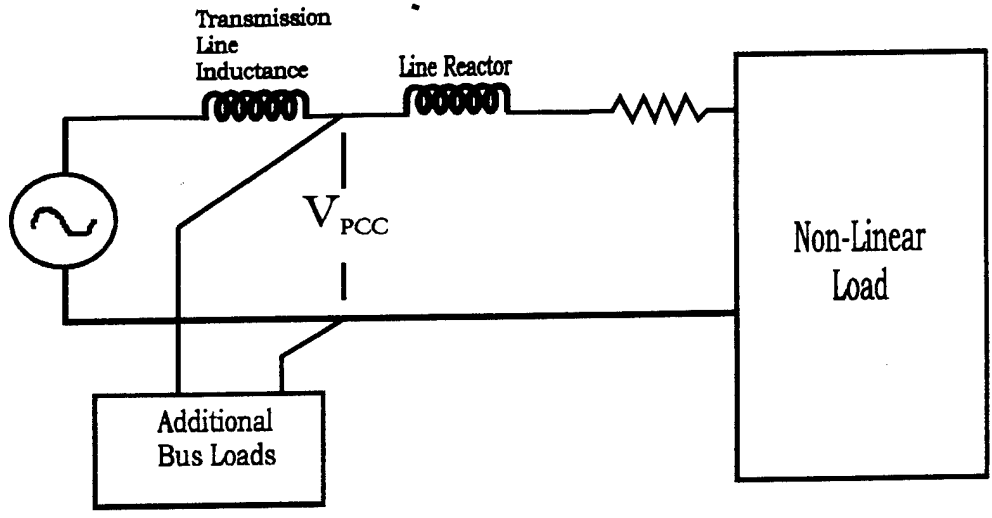
Figure 2.3 Line Reactor
