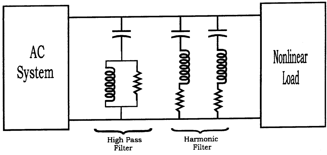
Figure 2.4 Custom Designed Harmonic Filter
