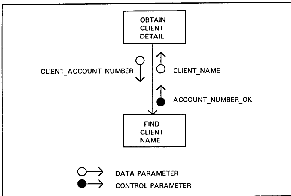
Figure 15. Module communications
