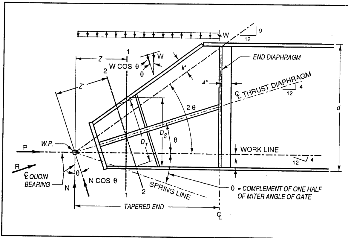
Figure 11. Tapered end critical section
