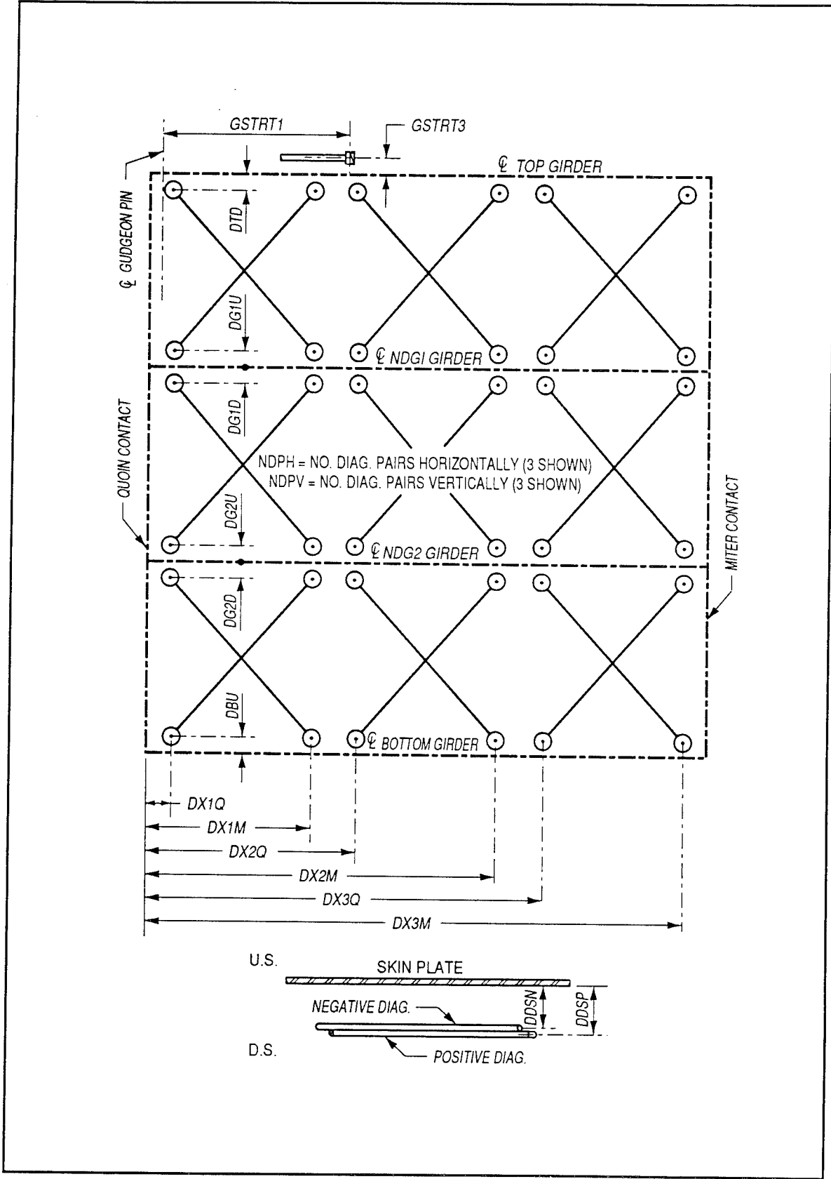
Figure 21. Group III, diagonals
