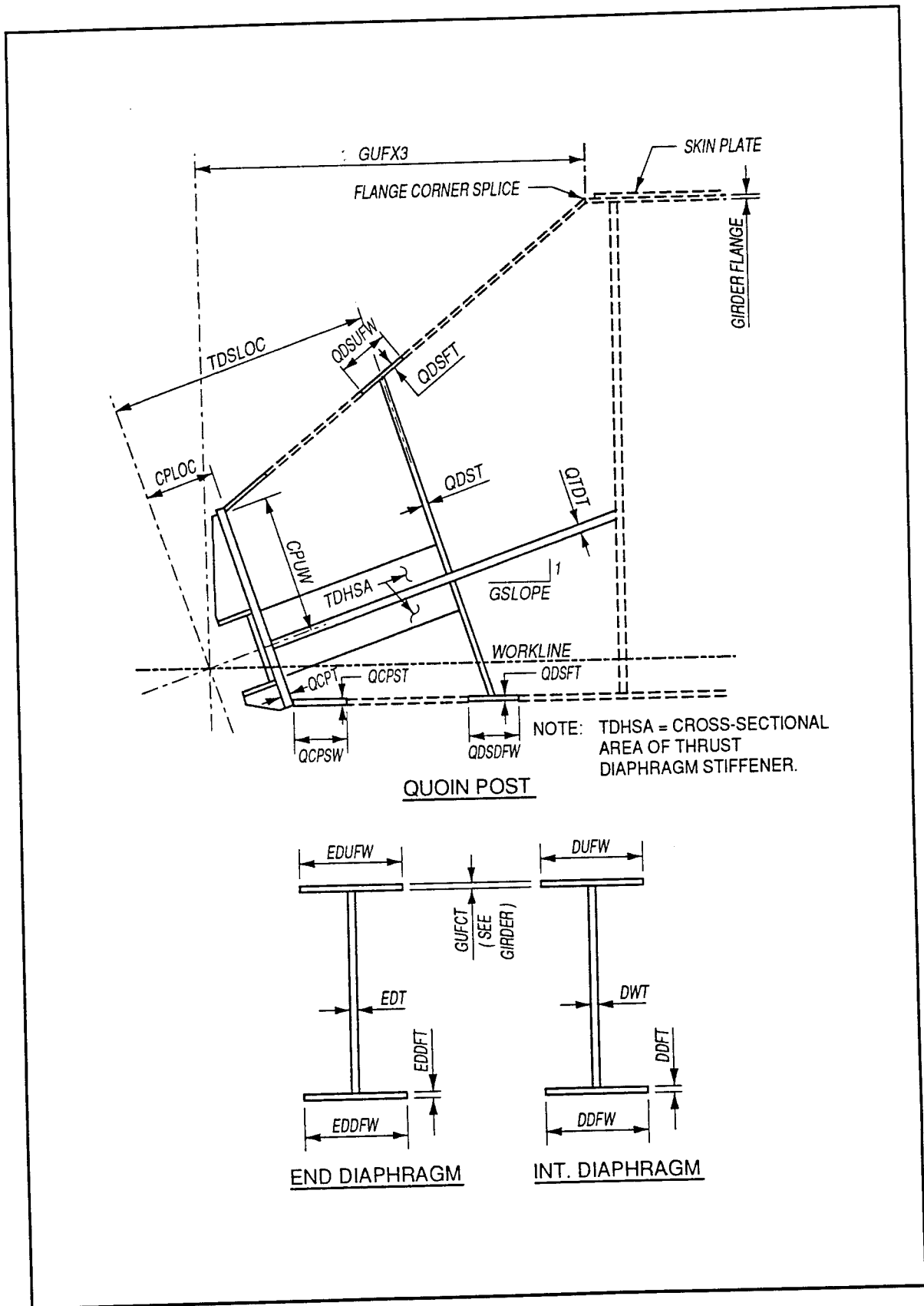
Figure 20. Group III, quoin, tapered end, and end diaphragm data
