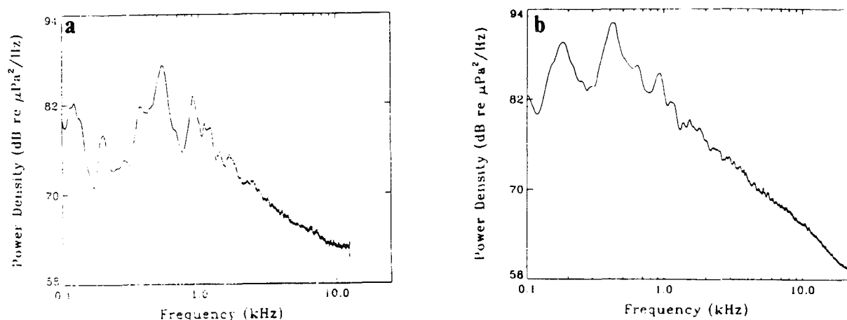
Figure 3. Power densities averaged over 100 acoustic signals generated by moderate spilling breakers. (a) Fresh water and (b) Salt water.
