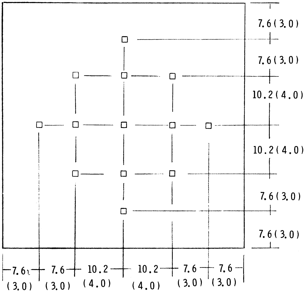
Figure 3.- Thermocouple locations in Lockalloy specimen. All dimensions are given in centimeters (inches).
