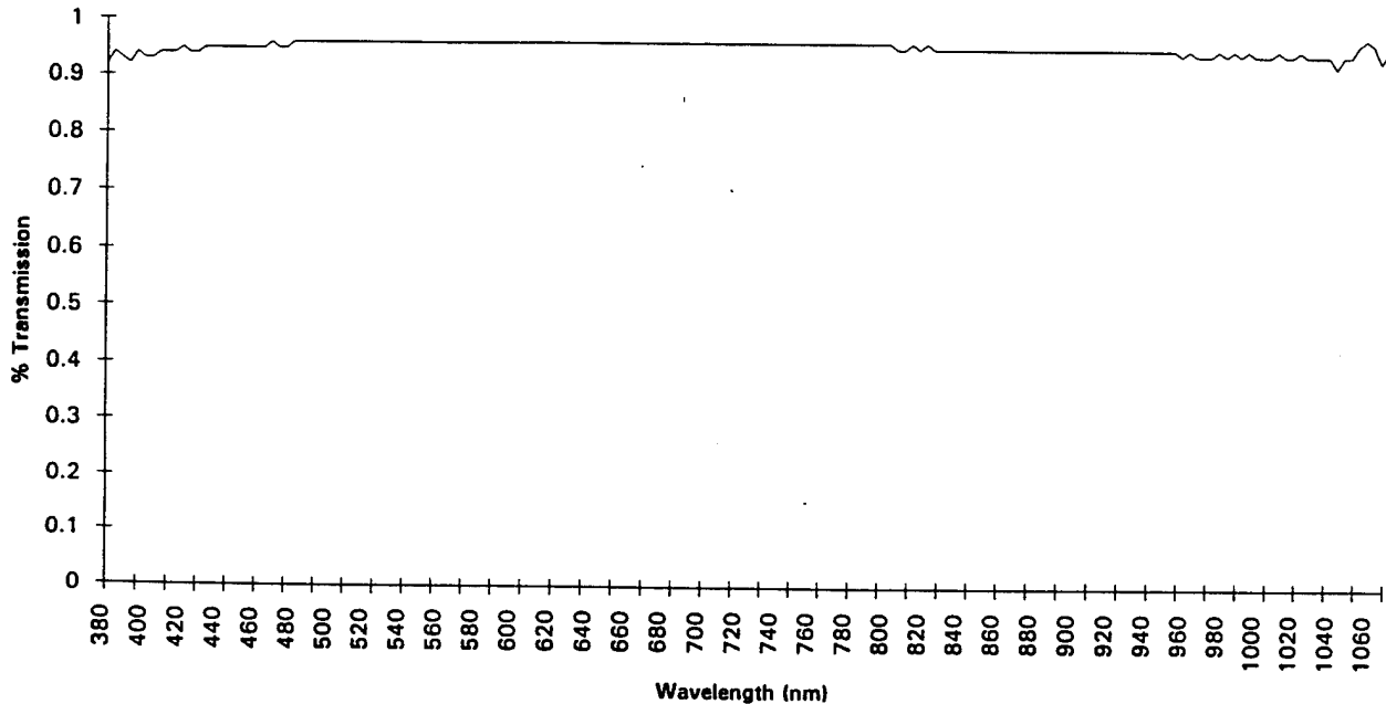
Figure 2 HUD TRANSMISSIVITY
