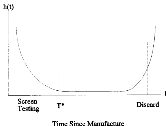
Figure 12. Bathtub Curve
