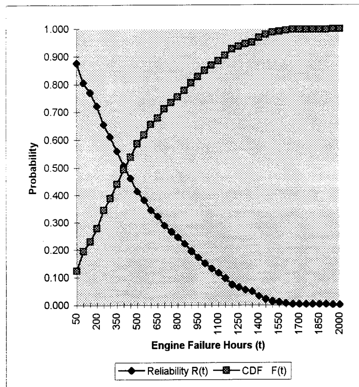
Figure 3. Non-parametric Statistical Functions Curves (Less zero failure times)
