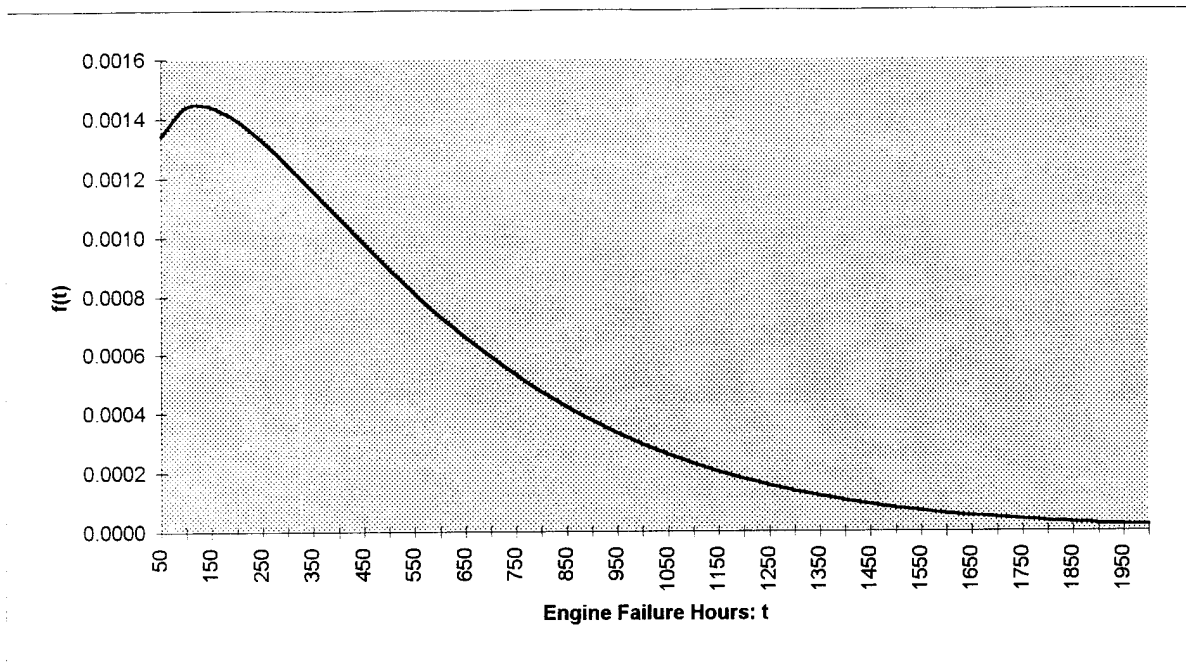
Figure 5. Weibull Distribution PDF (All failure times)
