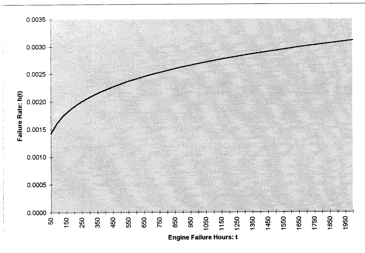
Figure 6. Weibull Distribution Failure Rate (All failure times)
