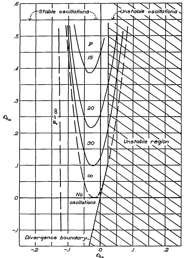
FIGURE 6.—Stability boundaries and lines of equal period for 15-percent-chord ailerons. \xi=0 ; I_a=0.0125 . Period P is in wing semispans.
