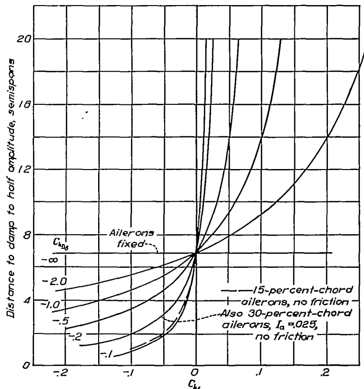
FIGURE 10.—Damping of the oscillations measured by the distance required to damp to half amplitude, in wing semispans, for ailerons with various values of C_{h\delta} . Mass-balanced ailerons, I_a=0.0125 ; \frac{C_{l\beta}}{I_x}=-0.4 .
