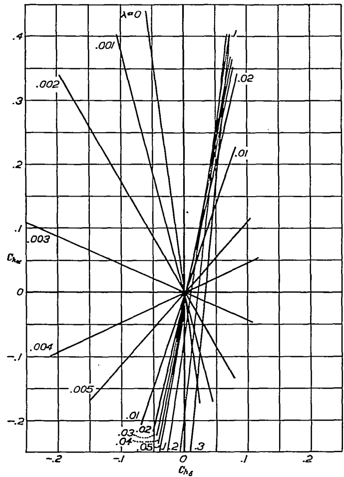
FIGURE 3.—Rate of divergence, as indicated by the value of the positive real roots of the stability equation. Aileron chord, 15-percent airfoil chord; \xi=0 ; I_\alpha=0 ; dihedral angle, 5^\circ ; C_L=1.0 .
