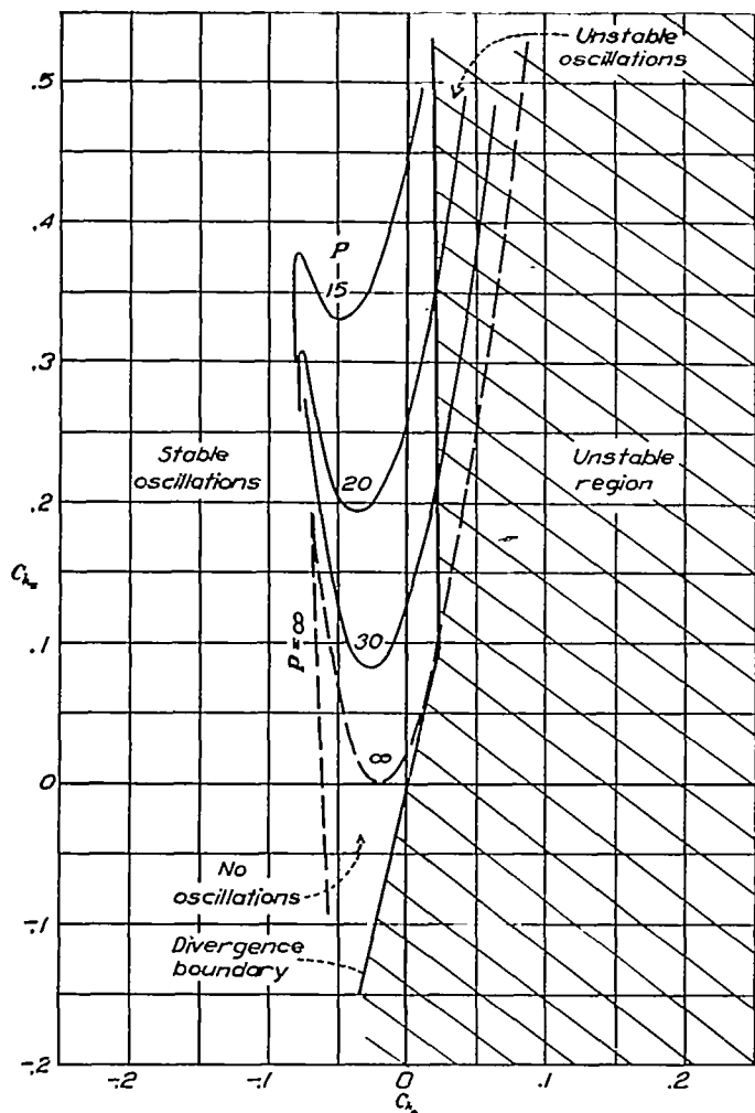
FIGURE 7.—Stability boundaries and lines of equal period for 15-percent-chord ailerons. \xi=0 ; I_a=0.025 . Period P is in wing semispans.
