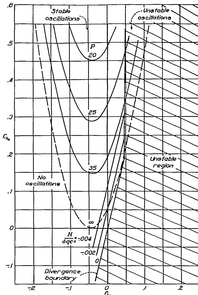
FIGURE 8.—Stability boundaries, lines of equal period, and lines of equal stick force for 30-percent-chord ailerons. \xi=0 ; I_a=0 . Period P is in wing semispans.
