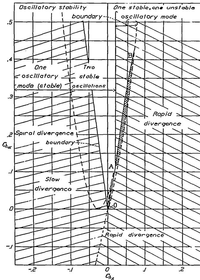
FIGURE 2.—Character and stability of the components of the motions found by solution of the equations before the elimination of sideslipping and yawing. (Shading indicates the unstable region.) Aileron chord, 15-percent airfoil chord; \xi=0 ; I_\alpha=0 ; dihedral angle, 5^\circ ; C_L=1.0 .
