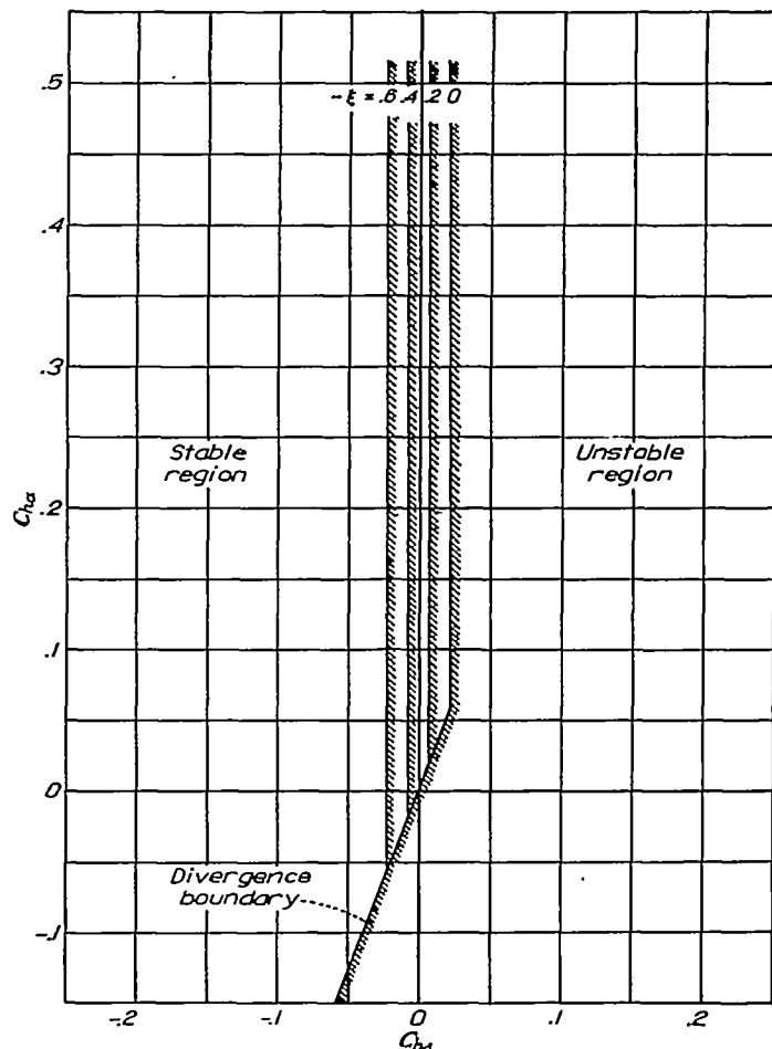
FIGURE 11.—Stability boundaries for 15-percent-chord ailerons, showing the effect of variation in the mass-moment parameter \xi . I_a=0.0125 ; C_{h\delta}=-0.011 .
