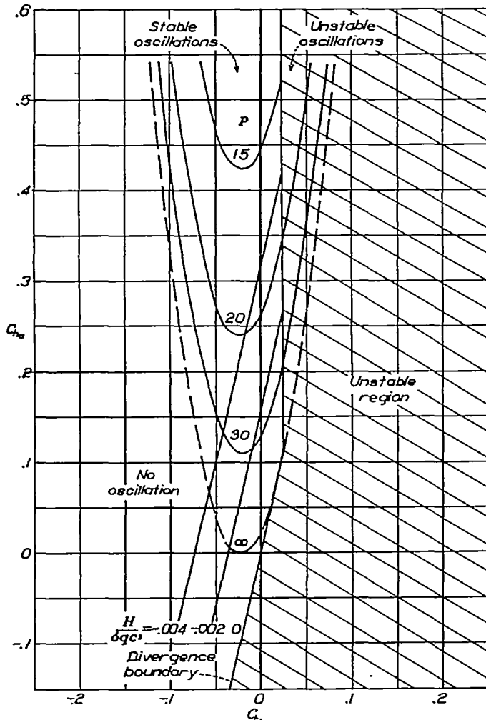
FIGURE 5.—Stability boundaries, lines of equal period, and lines of equal stick force for 15-percent-chord ailerons. \xi=0 ; I_a=0 . Period P is in wing semispans.
