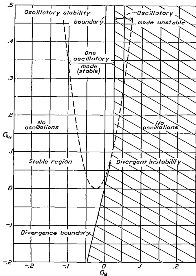
FIGURE 4.—Character and stability of the components of the motions with coupling only between aileron movements and rolling angle. Aileron chord, 15-percent airfoil chord; \xi=0 ; I_a=0 .
