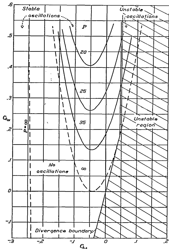
FIGURE 9.—Stability boundaries and lines of equal period for 30-percent-chord ailerons. \xi=0 ; I_a=0.025 . Period P is in wing semispans.
