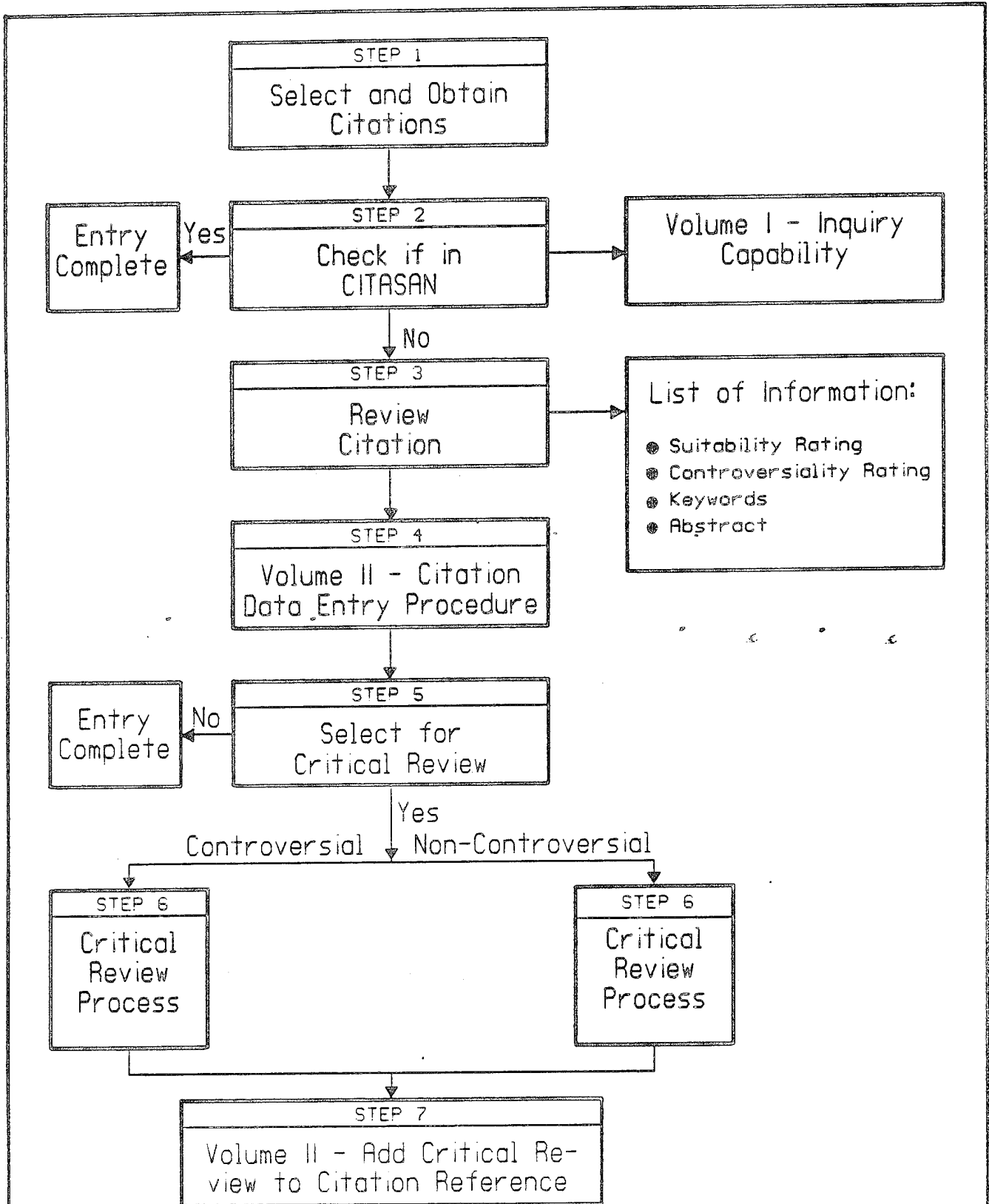
FIGURE 1. BLOCK DIAGRAM OF THE GENERAL PROCESS FOR ADDING NEW CITATIONS TO CITASAN
