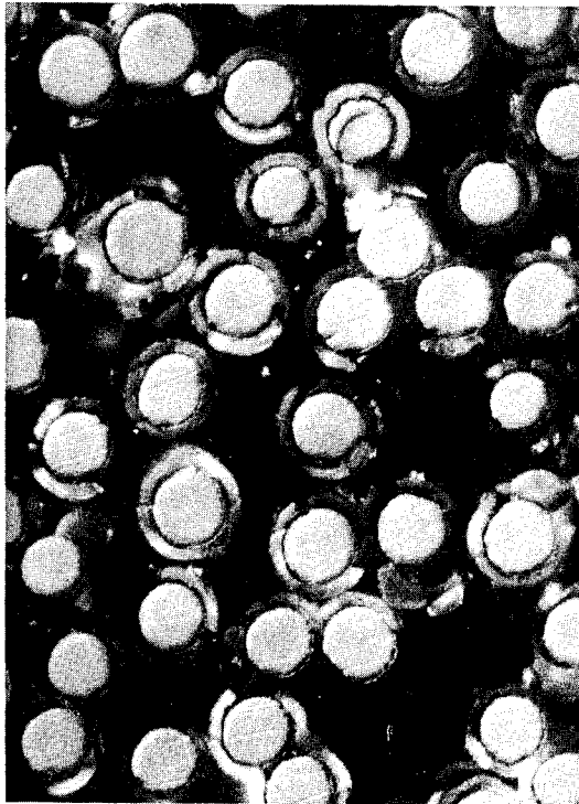
Fig. 28 CVD \text{Si}_3\text{N}_4 Coated Celion 6000 Yarn
