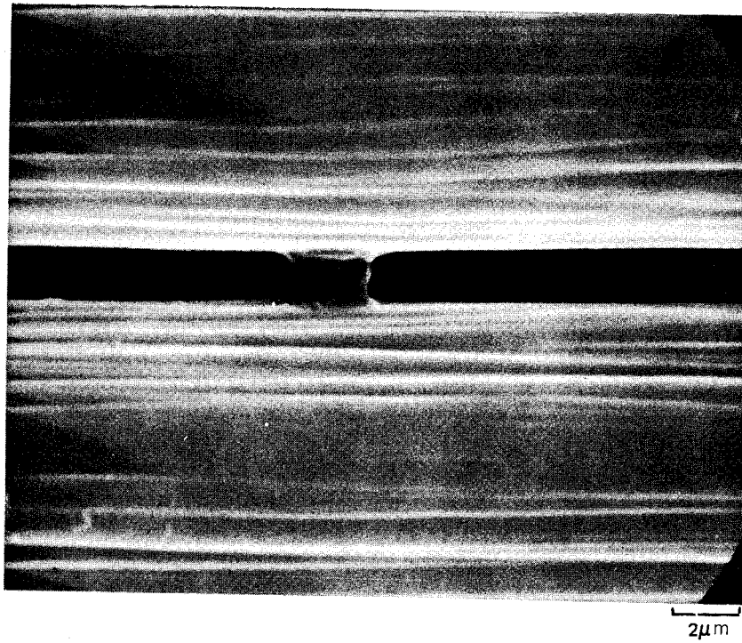
Fig. 19 SEM of Silicon Nitride Coated HTS Graphite Yarn
