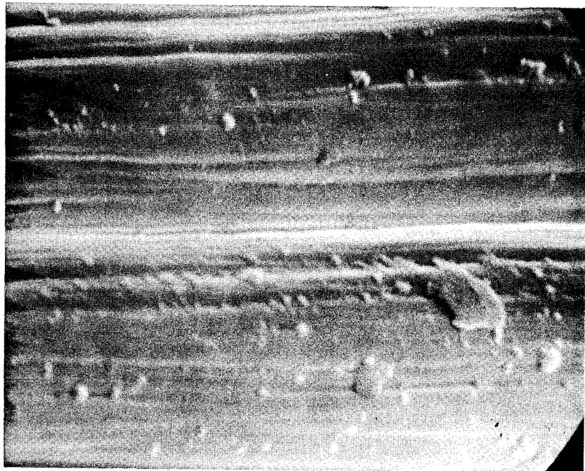
Fig. 16 SEM of Silicon Nitride Coated HTS Graphite Yarn
