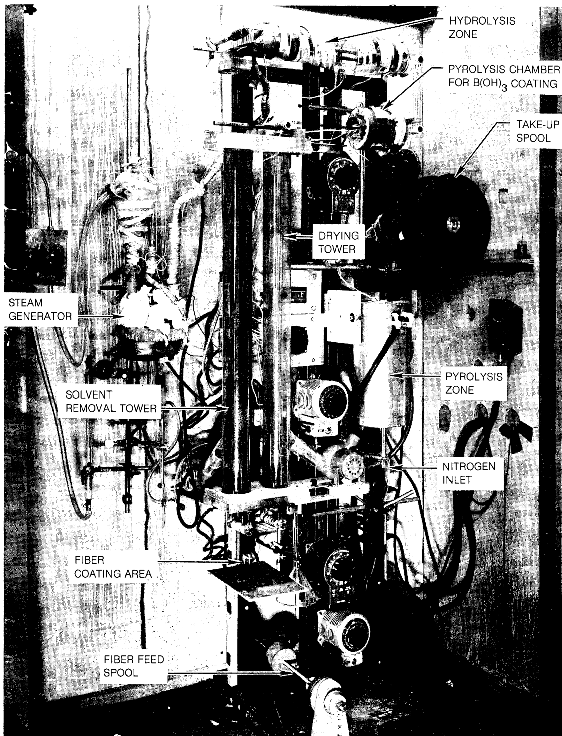
Fig. 6 Modified Continuous Fiber Coating Apparatus
