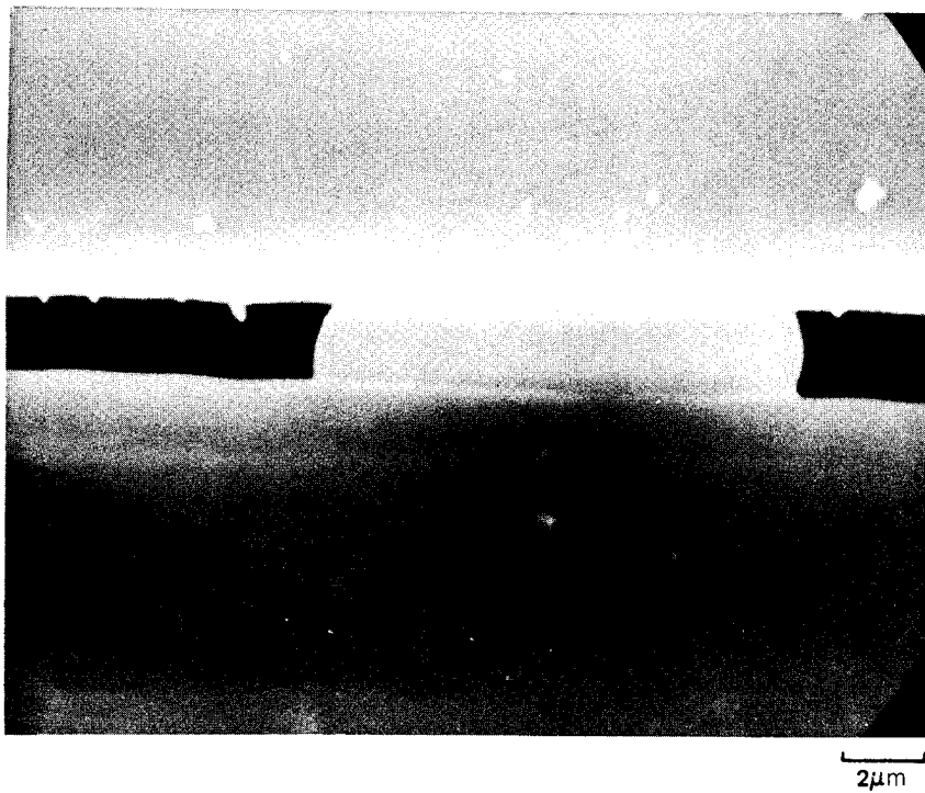
Fig. 15 SEM of Silicon Nitride Coated HTS Graphite Yarn
