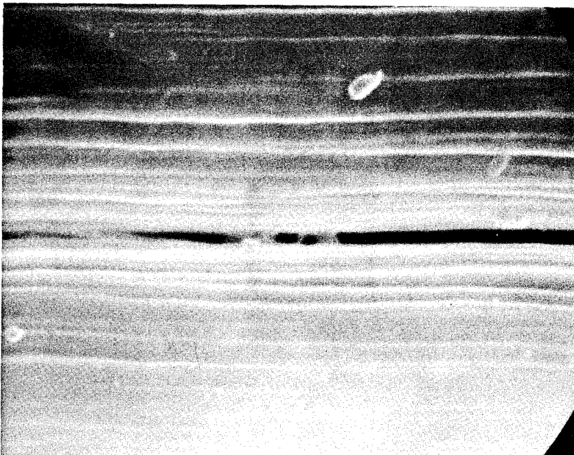
Fig. 17 SEM of Silicon Nitride Coated HTS Graphite Yarn
