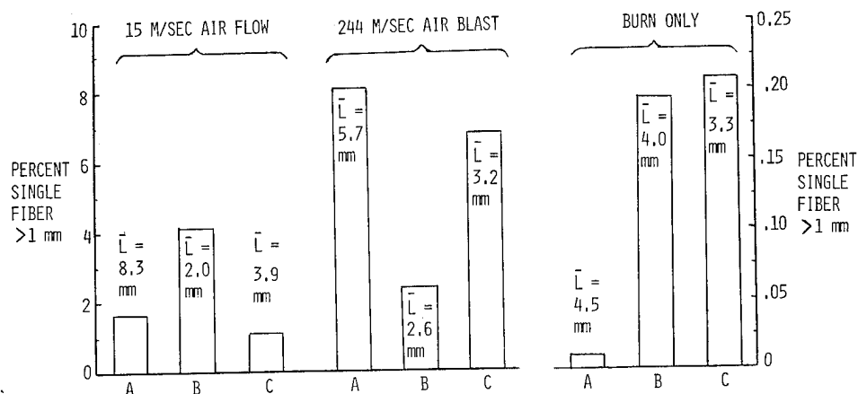
Figure 7.- Release of single carbon fibers from carbon fiber/NOMEX honeycomb panels under different test conditions. A-Panel skins: 2 plies of carbon tape ( 0 + 90^\circ ) with fiberglass scrim. B-Panel skins: 2 plies of carbon fabric. C-Panel skins: 1 ply of carbon fabric and 1 ply of Kevlar fabric. \bar{L} = mean fiber length.
