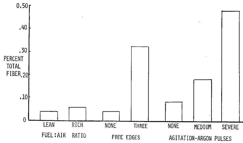
Figure 9.- Effects of fire variables on total carbon fiber release.
