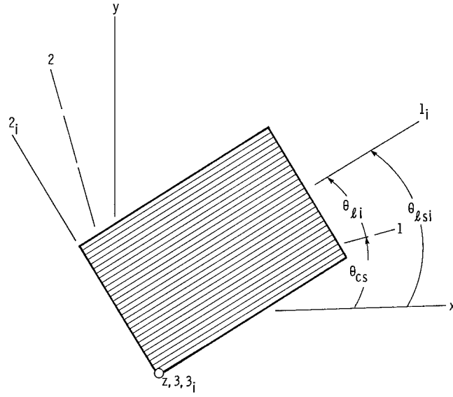
Figure 6.—Ply orientation geometry. Composite structural axes, x, y, z ; composite material axes, 1, 2, 3 ; ply material axes (coincides with fiber direction), 1_l, 2_l, 3_l .
