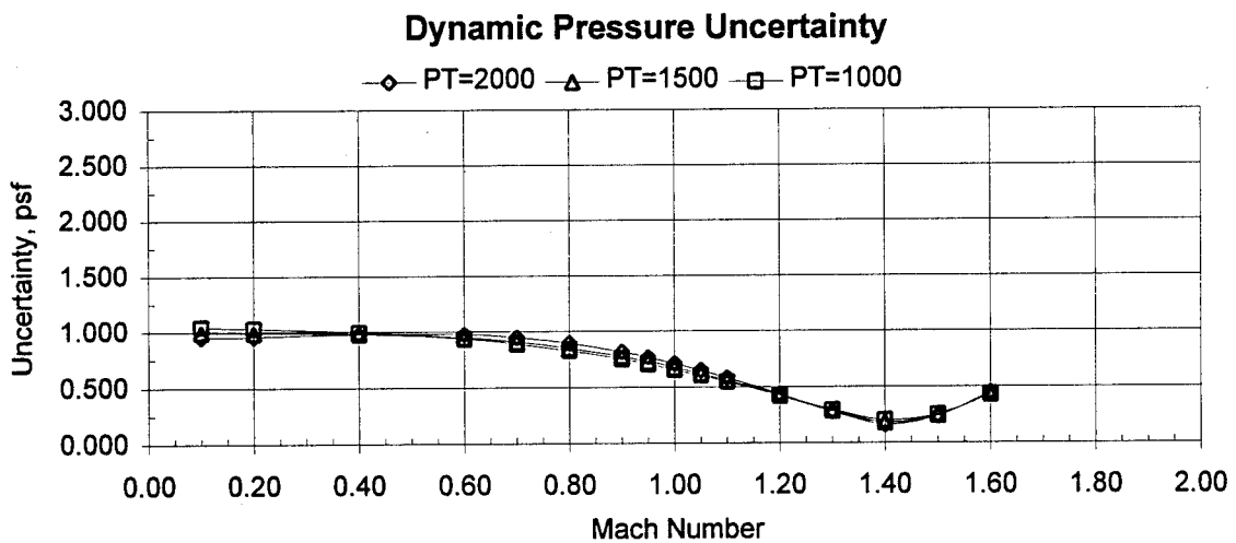
Figure 3. Estimated Uncertainties in 16T Tunnel Parameters
