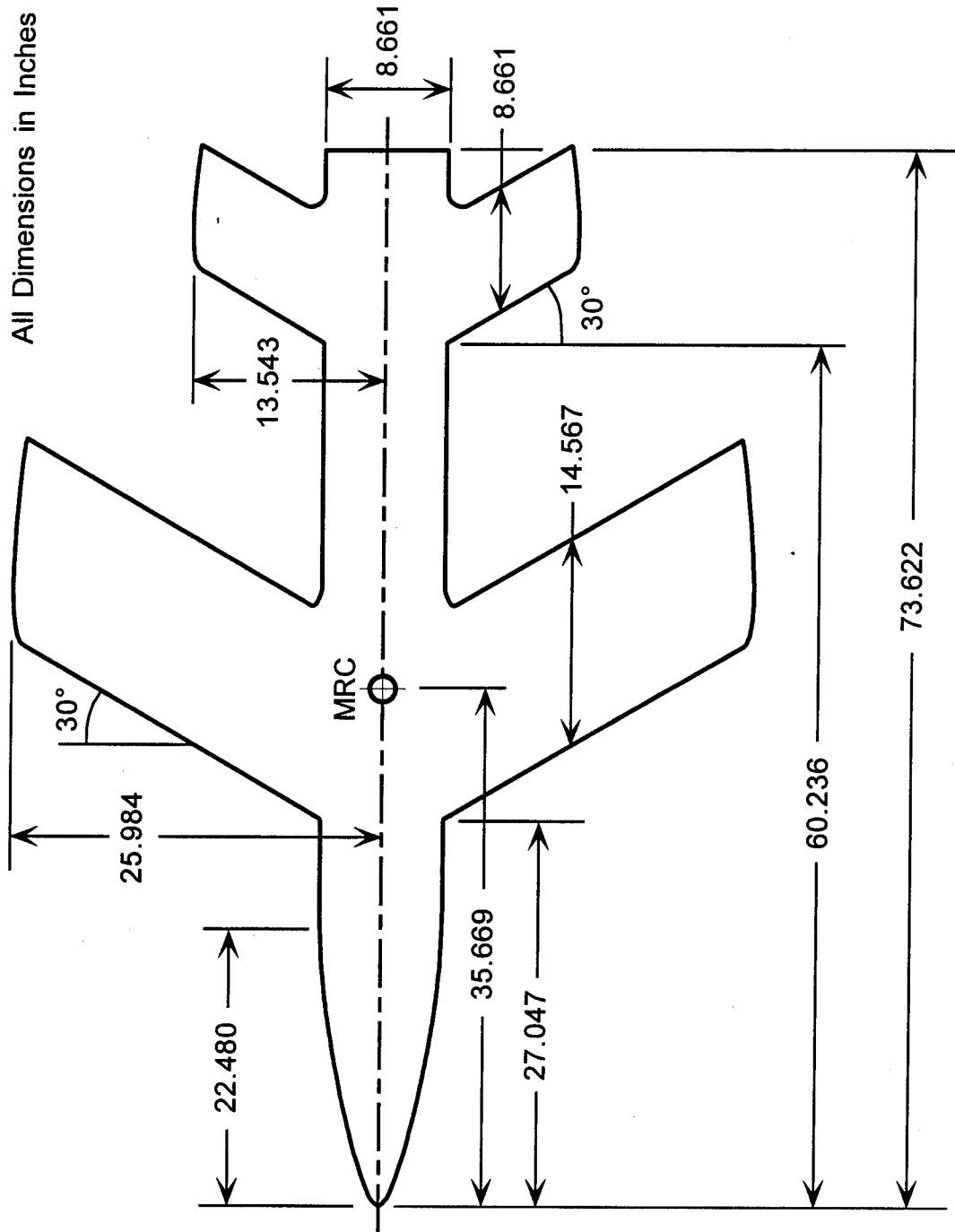
Figure 2. Model Details
