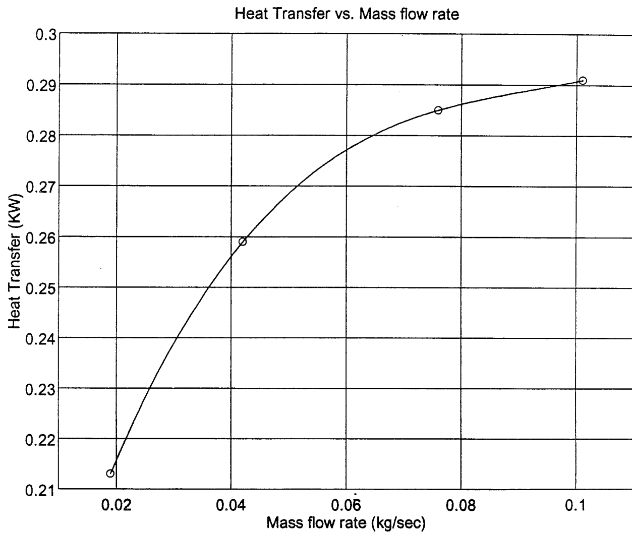
Figure 12: Graphical representation of Heat Transfer with mass flow rate.
