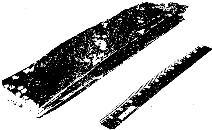
UN-DEBULKED LAYUP
