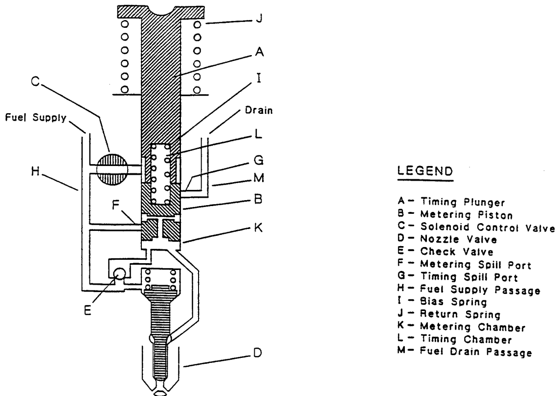
Figure VII-7. ECI injector schematic
