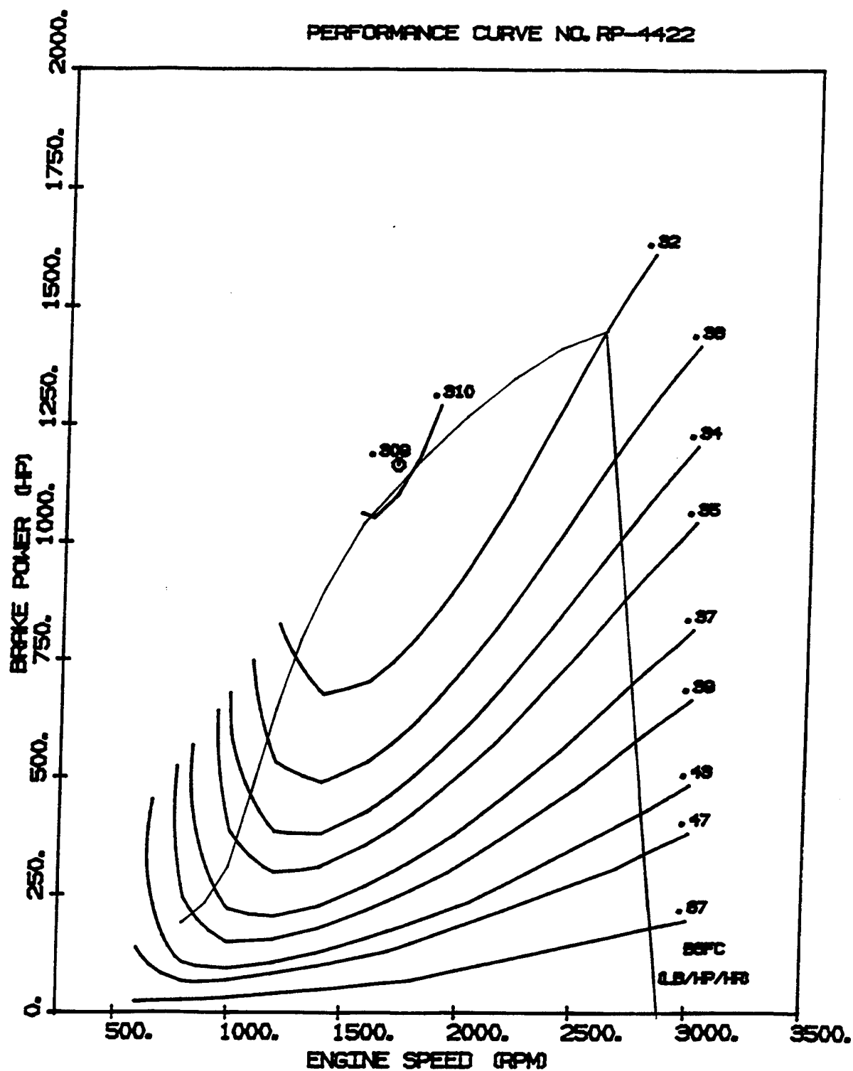
Figure VII-5. dAIPS fuel map
