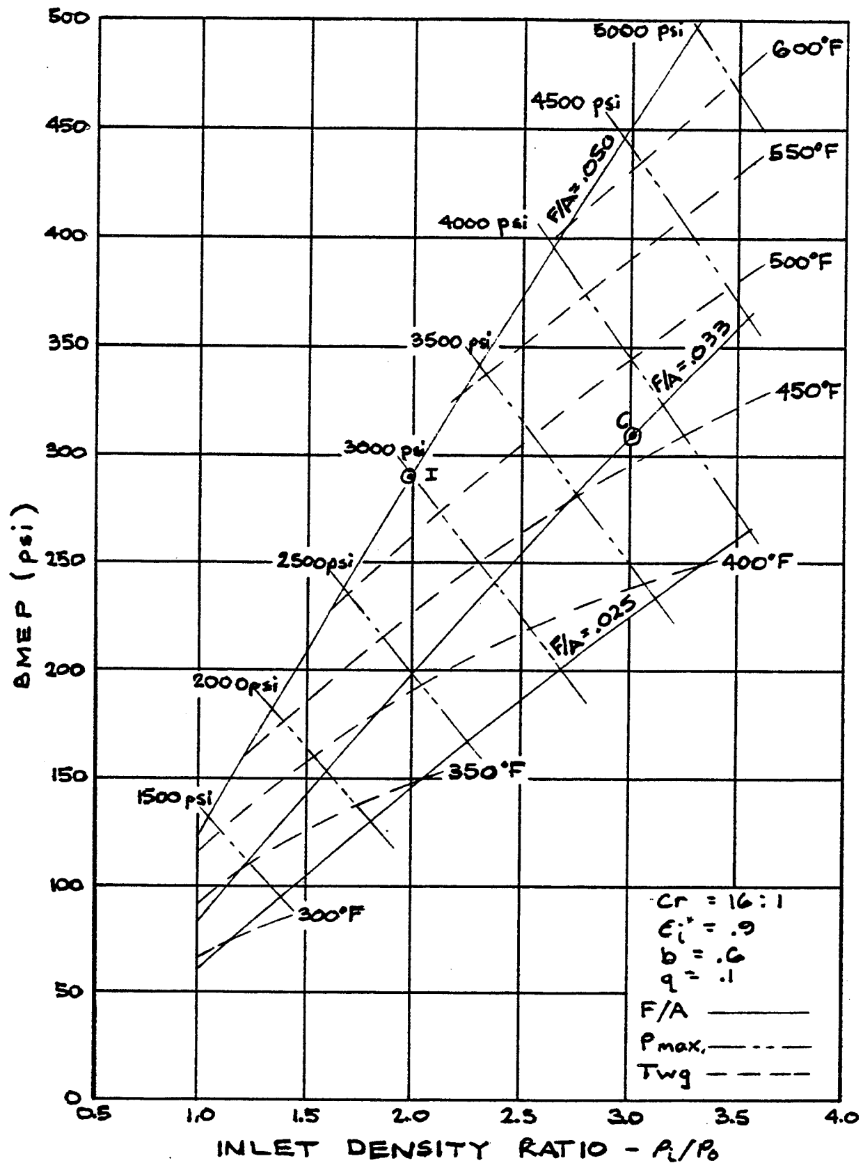
Figure IX-3. CR = 16, high aftercooling
