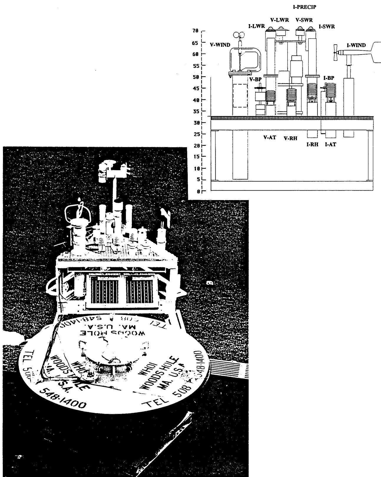
Figure 4. Discus buoy with fully instrumented tower top.
