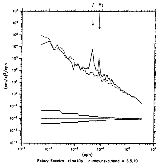
Figure 16. Northeast and central separate deployment spectra.
