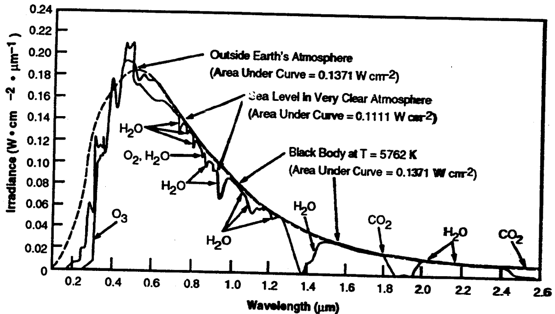
Figure 6-3. Normally incident solar radiation at sea level on very clear days, solar spectral irradiance outside the Earth's atmosphere at 1 AU, and blackbody spectral irradiance curve at T = 5762 K (normalized to 1 AU).
