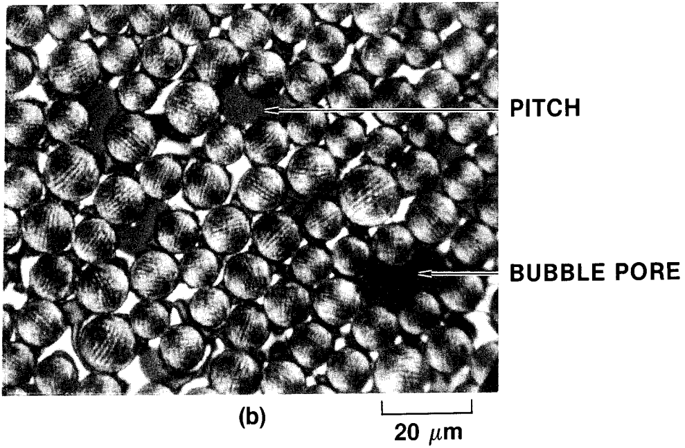
Figure 8. Fiber Bundle in a Pressure-cycled Specimen. From Fig. 7b, a fiber bundle adjacent to a poorly filled weave cavity. Partially crossed polarizers.
