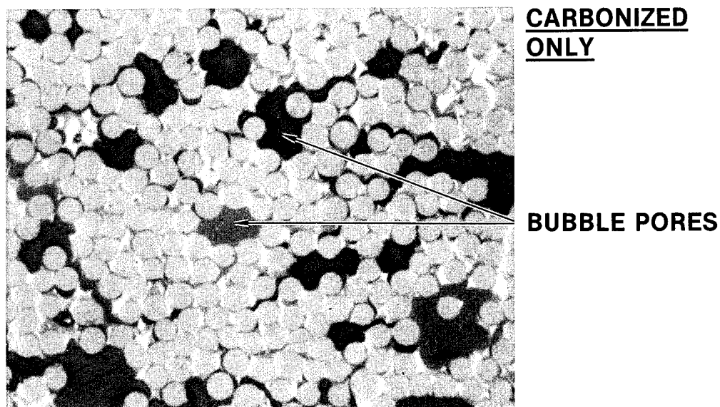
Figure 15. Microstructures of Mesophase Matrices after Carbonization. High-magnification views of specimens in Figs. 13 and 14: Top: carbonized after oxidation; mesophase-pitch wetting conditions are retained; crossed polarizers, oil immersion. Bottom: carbonized without oxidation; polarizer only. Oil immersion.
