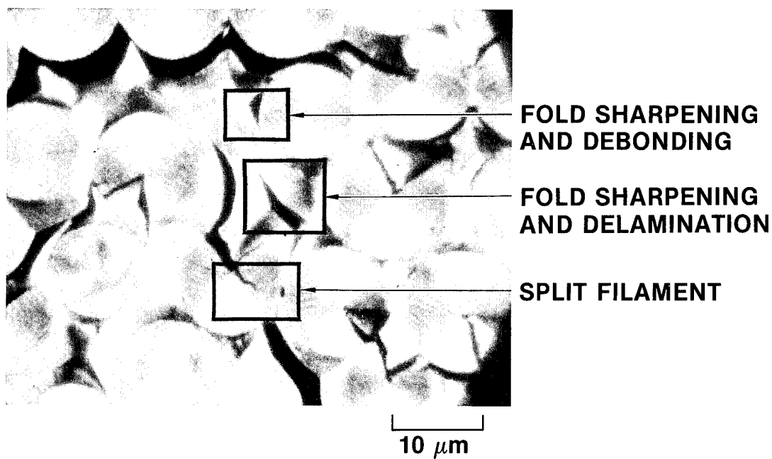
Figure 20. Mesophase Shrinkage, Distortion, and Debonding from Filaments in a Fiber Bundle Heat-treated to 1680°C. Transverse views of a unidirectional composite prepared by high-pressure pyrolysis of VSA-11 mesophase carbon fiber impregnated with A240 petroleum pitch. Polarized light, oil immersion.
