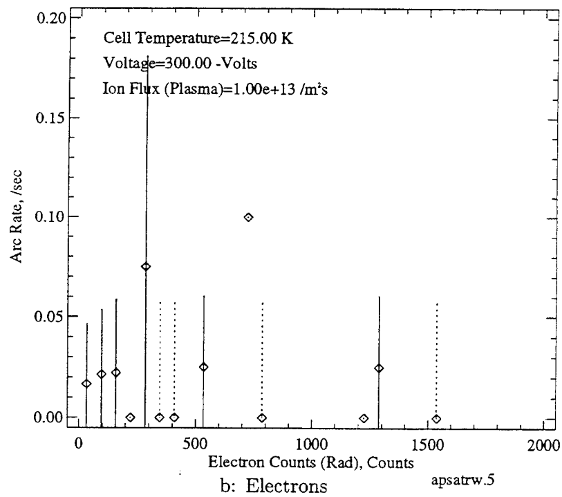
Figure 76: Arc Rate Variation with Radiation Flux for APSA Module #5
