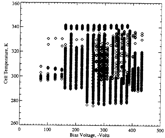
b: Voltage/Cell Temperature Data Space for Mini-Cassegrainian Module 14
