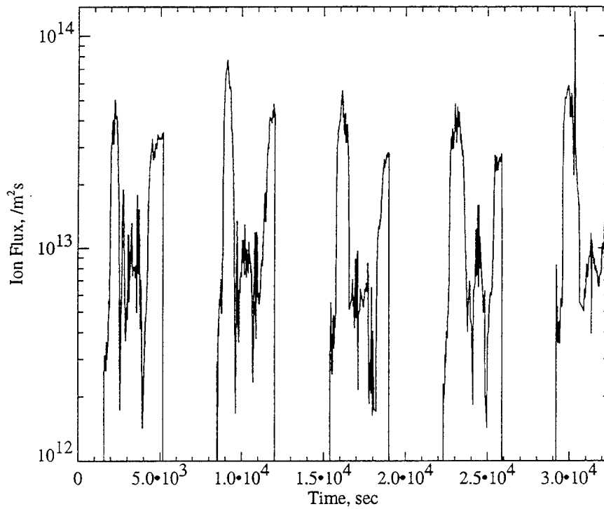
Figure 29: PASP Plus Ion Flux During Five Orbits on Day 94235
