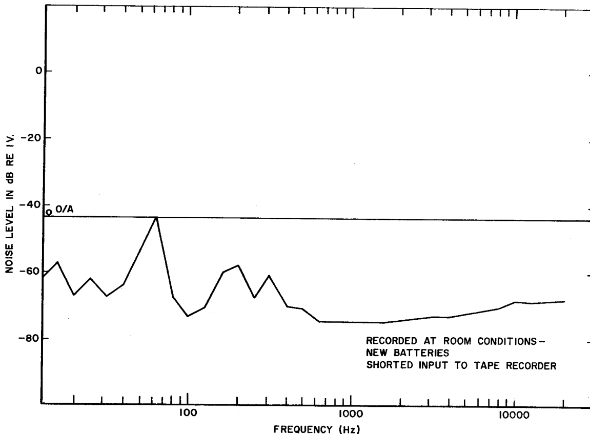
Fig. 8. Noise Floor of Tape Recorder
