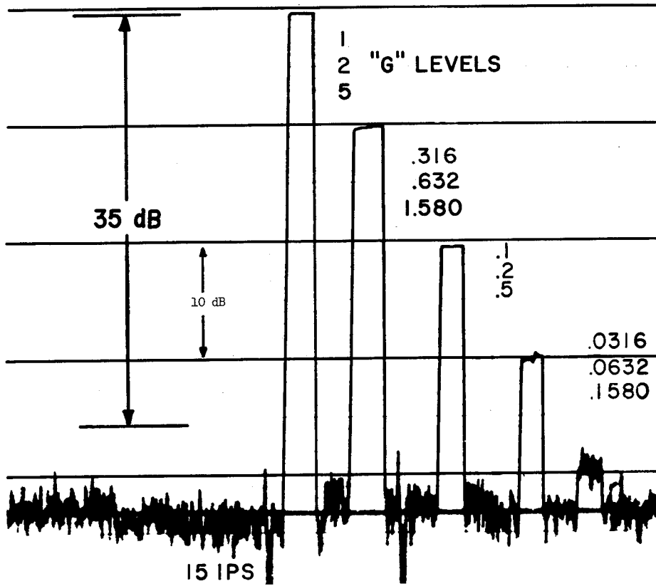
Fig. 6B. Characteristics of the Vibration Recording Section — Dynamic Ranges for 3 Different Acceleration Levels
