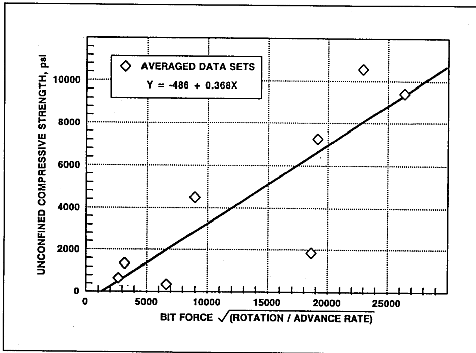
Figure 5. DPR drilling test correlation with UCS
