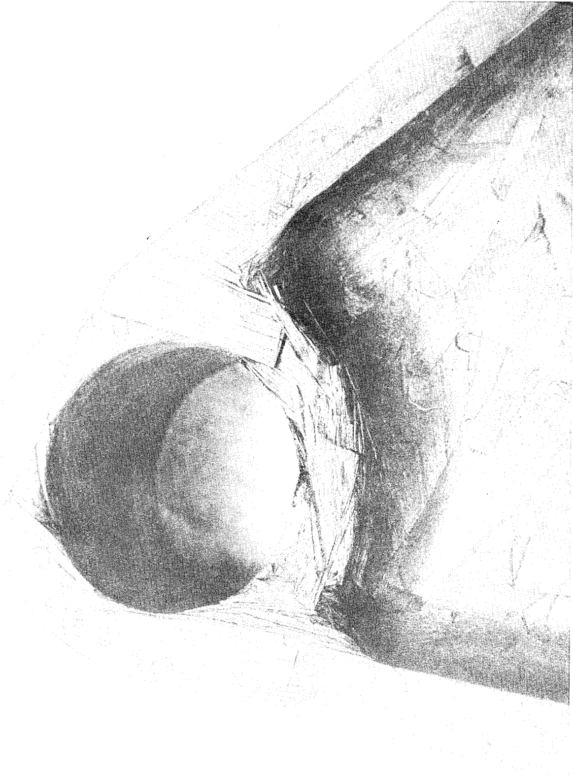
Figure 16. Poor Flow and Mold Conformance of Molding Compound Imidized at 204°C (400°F)
