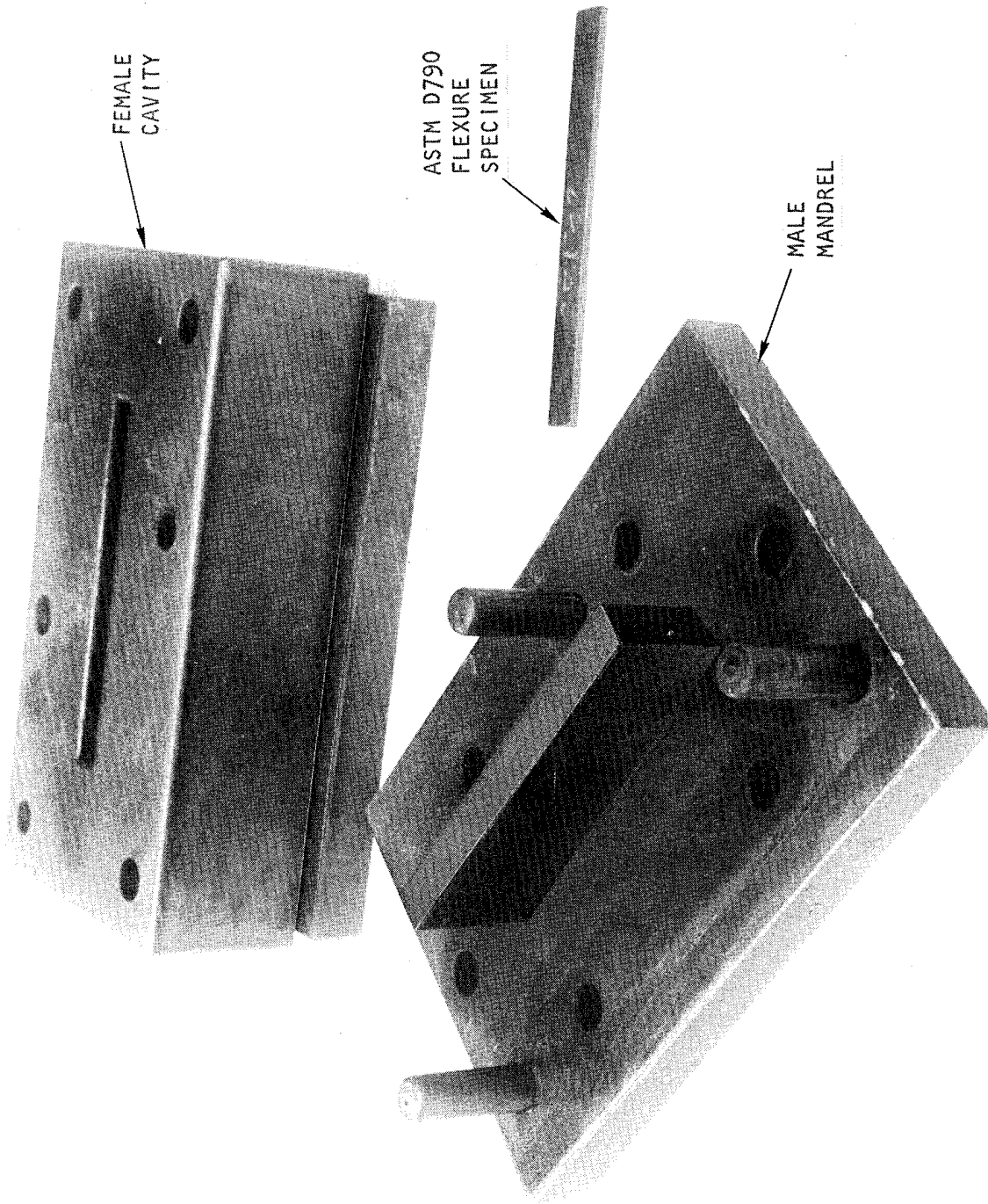
Figure 11. ASTM D 647 Compression Mold for Celion/LARC 160 Molding Compound Flexure Specimen per ASTM D 790
