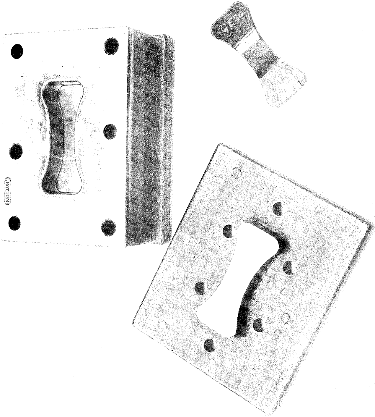
Figure 12. ASTM D647 Tensile Mold and Molded ASTM D651 Tension Coupon
