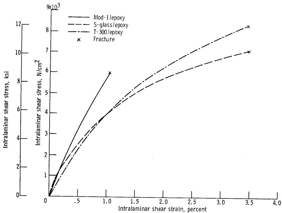
Figure 8. - Intralaminar shear stress-strain diagrams for three materials.
