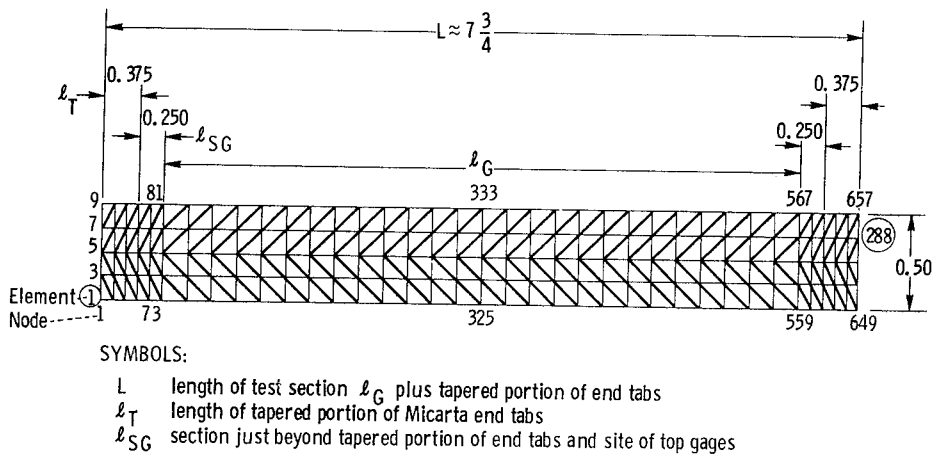
Figure 5. - Grid for finite element analysis of Mod-I/epoxy specimens. (Top gages located at nodes 74 and 77; midpoint gages located at nodes 326, 329, and 332. All dimensions shown are relative.)
