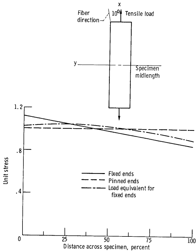
Figure 6. - Finite element analysis results of axial stress variation at midlength for three different boundary conditions; Mod-I/epoxy 10^0 off-axis tensile specimen. (See fig. 5 for finite element representation.)
