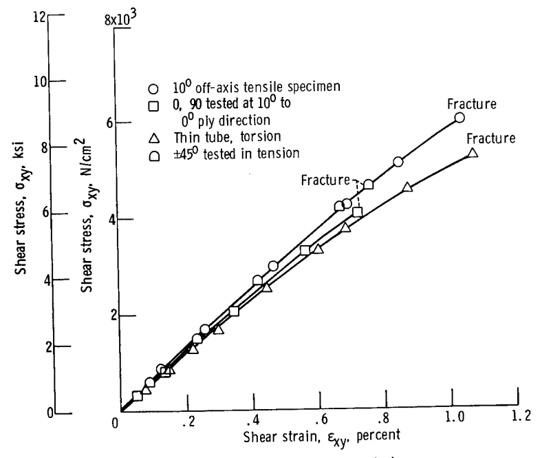
Figure 10. - Comparison of shear stress-strain curves.
