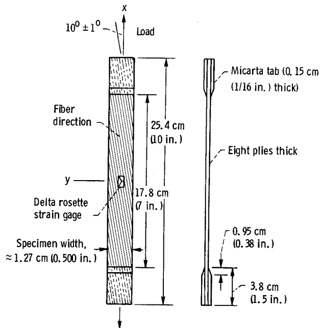
Figure 12. - Schematic showing geometry and instrumentation of proposed 10^0 off-axis tensile specimen for fiber composite intralaminar shear characterization.
