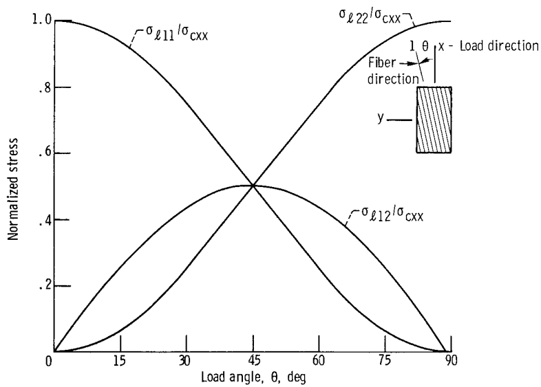
Figure 2. - Variation of material axes stress in unidirectional composite plotted against load direction.
