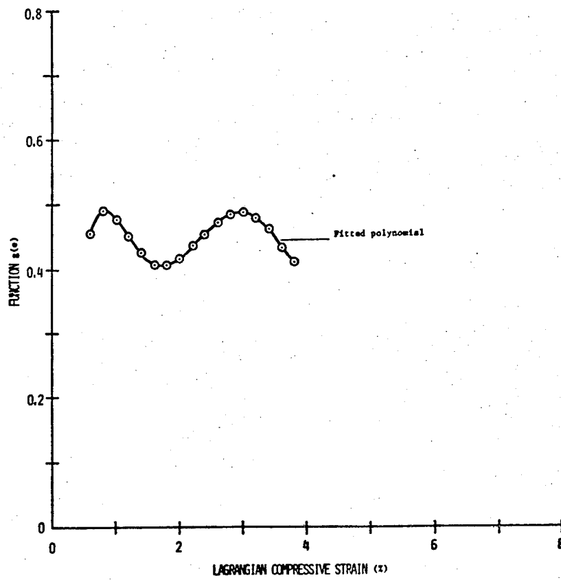
Figure 4.6 Function g(\epsilon) for tests LS2-17 and LS2-19
