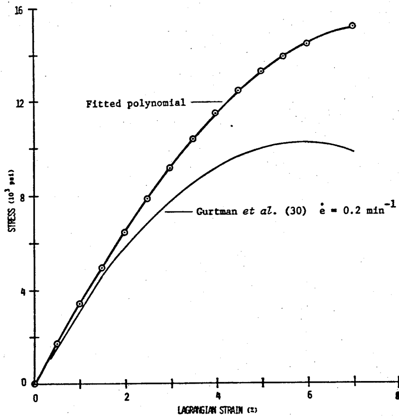
Figure 4.3 Dynamic stress-strain curve for Lexan at 72°F (curve is independent of strain rate in a range of strain rates from 300 sec -1 to 2000 sec -1 )
