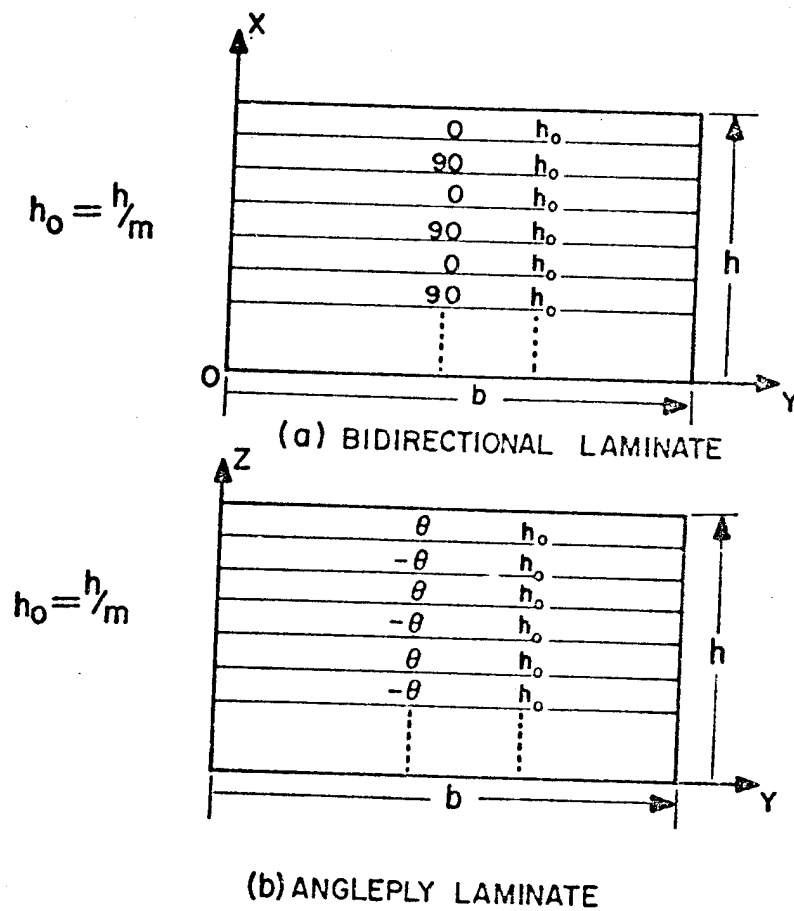
FIGURE 6. BIDIRECTIONAL AND ANGLE-PLY LAMINATES
