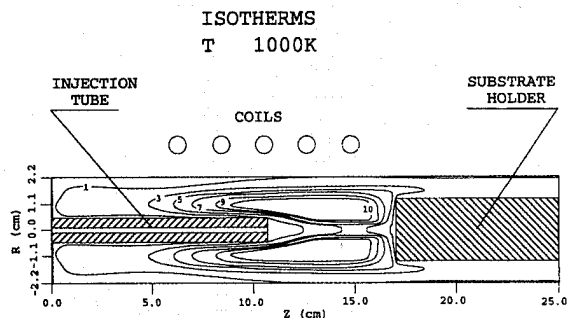
Temperature Distribution in a Diamond CVD Reactor
