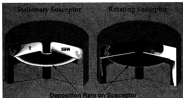
Effect of Susceptor Rotation on CVD of Silicon in a Radial Flow Reactor (CFD-ACE)
